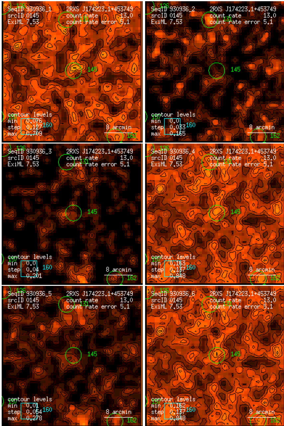
Figure 145: RASS 930936: detection 0145: band rate images, Gaussian filter: (1) PSPC channels 11 – 41, (2) 52 – 90, (3) 91 – 201, (4) 11 – 235, (5) 52 – 201, (6) 11 – 201. Broad band rates in counts/ks. Band rate contour levels in counts/ks/arcmin 2 .
