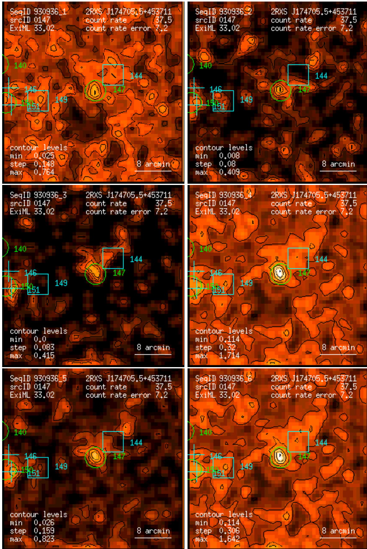
Figure 147: RASS 930936: detection 0147: band rate images, Gaussian filter: (1) PSPC channels 11 – 41, (2) 52 – 90, (3) 91 – 201, (4) 11 – 235, (5) 52 – 201, (6) 11 – 201. Broad band rates in counts/ks. Band rate contour levels in counts/ks/arcmin 2 .
