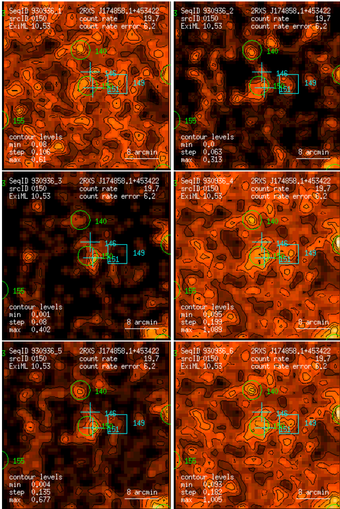
Figure 150: RASS 930936: detection 0150: band rate images, Gaussian filter: (1) PSPC channels 11 – 41, (2) 52 – 90, (3) 91 – 201, (4) 11 – 235, (5) 52 – 201, (6) 11 – 201. Broad band rates in counts/ks. Band rate contour levels in counts/ks/arcmin 2 .
