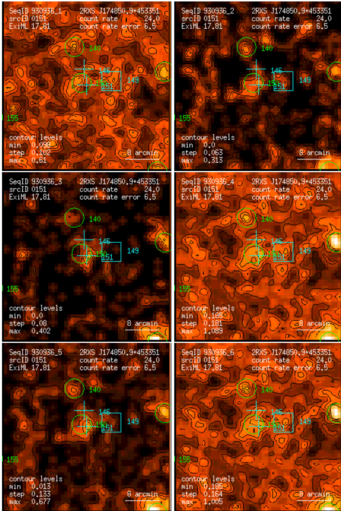
Figure 151: RASS 930936: detection 0151: band rate images, Gaussian filter: (1) PSPC channels 11 – 41, (2) 52 – 90, (3) 91 – 201, (4) 11 – 235, (5) 52 – 201, (6) 11 – 201. Broad band rates in counts/ks. Band rate contour levels in counts/ks/arcmin 2 .
