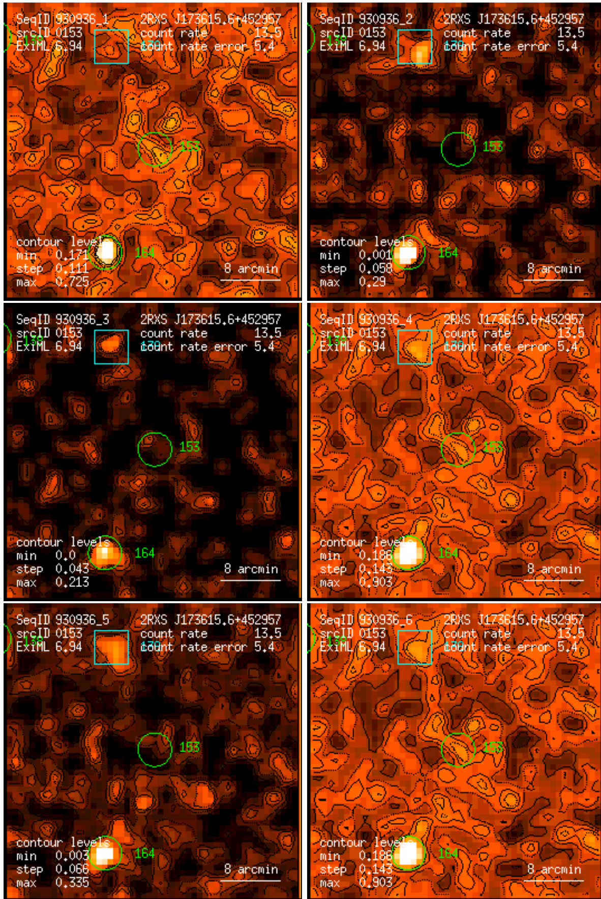
Figure 153: RASS 930936: detection 0153: band rate images, Gaussian filter: (1) PSPC channels 11 – 41, (2) 52 – 90, (3) 91 – 201, (4) 11 – 235, (5) 52 – 201, (6) 11 – 201. Broad band rates in counts/ks. Band rate contour levels in counts/ks/arcmin 2 .
