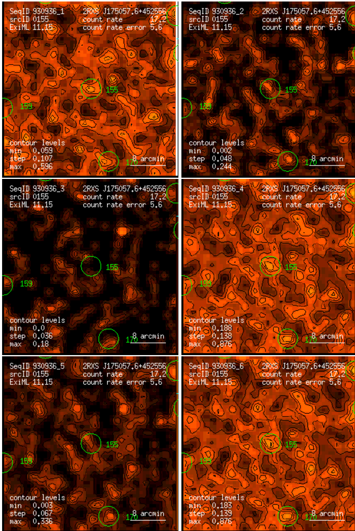
Figure 155: RASS 930936: detection 0155: band rate images, Gaussian filter: (1) PSPC channels 11 – 41, (2) 52 – 90, (3) 91 – 201, (4) 11 – 235, (5) 52 – 201, (6) 11 – 201. Broad band rates in counts/ks. Band rate contour levels in counts/ks/arcmin 2 .
