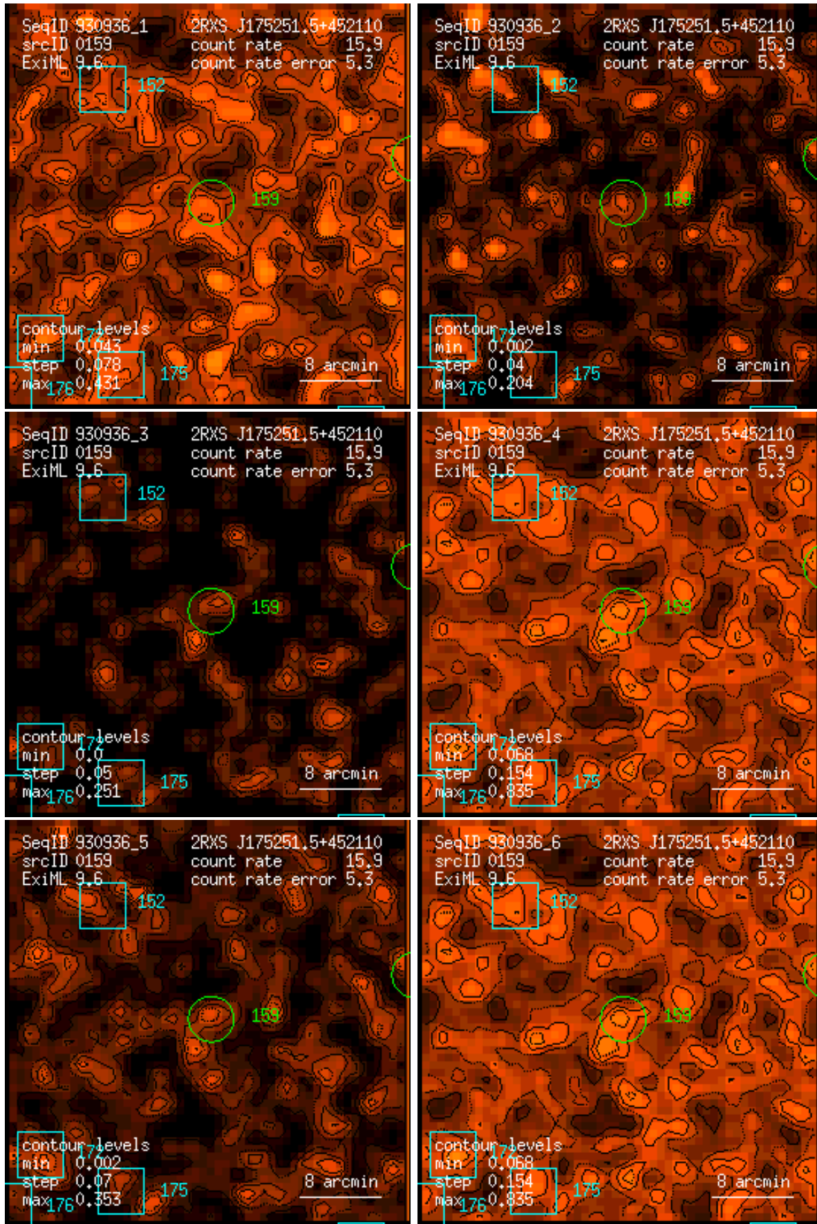
Figure 159: RASS 930936: detection 0159: band rate images, Gaussian filter: (1) PSPC channels 11 – 41, (2) 52 – 90, (3) 91 – 201, (4) 11 – 235, (5) 52 – 201, (6) 11 – 201. Broad band rates in counts/ks. Band rate contour levels in counts/ks/arcmin 2 .
