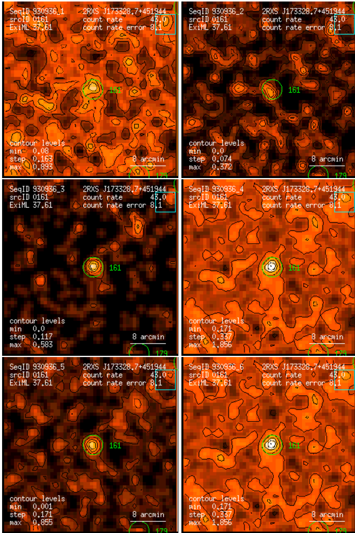
Figure 161: RASS 930936: detection 0161: band rate images, Gaussian filter: (1) PSPC channels 11 – 41, (2) 52 – 90, (3) 91 – 201, (4) 11 – 235, (5) 52 – 201, (6) 11 – 201. Broad band rates in counts/ks. Band rate contour levels in counts/ks/arcmin 2 .
