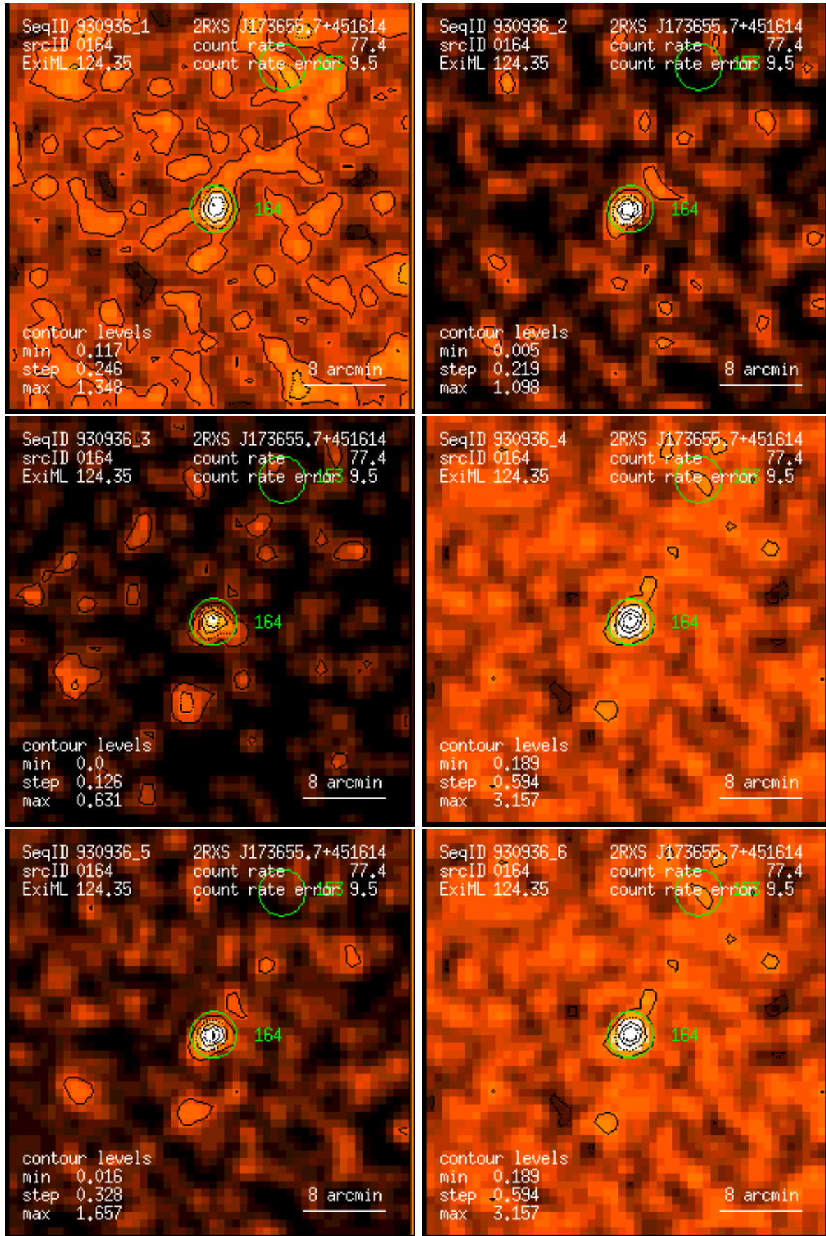
Figure 164: RASS 930936: detection 0164: band rate images, Gaussian filter: (1) PSPC channels 11 – 41, (2) 52 – 90, (3) 91 – 201, (4) 11 – 235, (5) 52 – 201, (6) 11 – 201. Broad band rates in counts/ks. Band rate contour levels in counts/ks/arcmin 2 .
