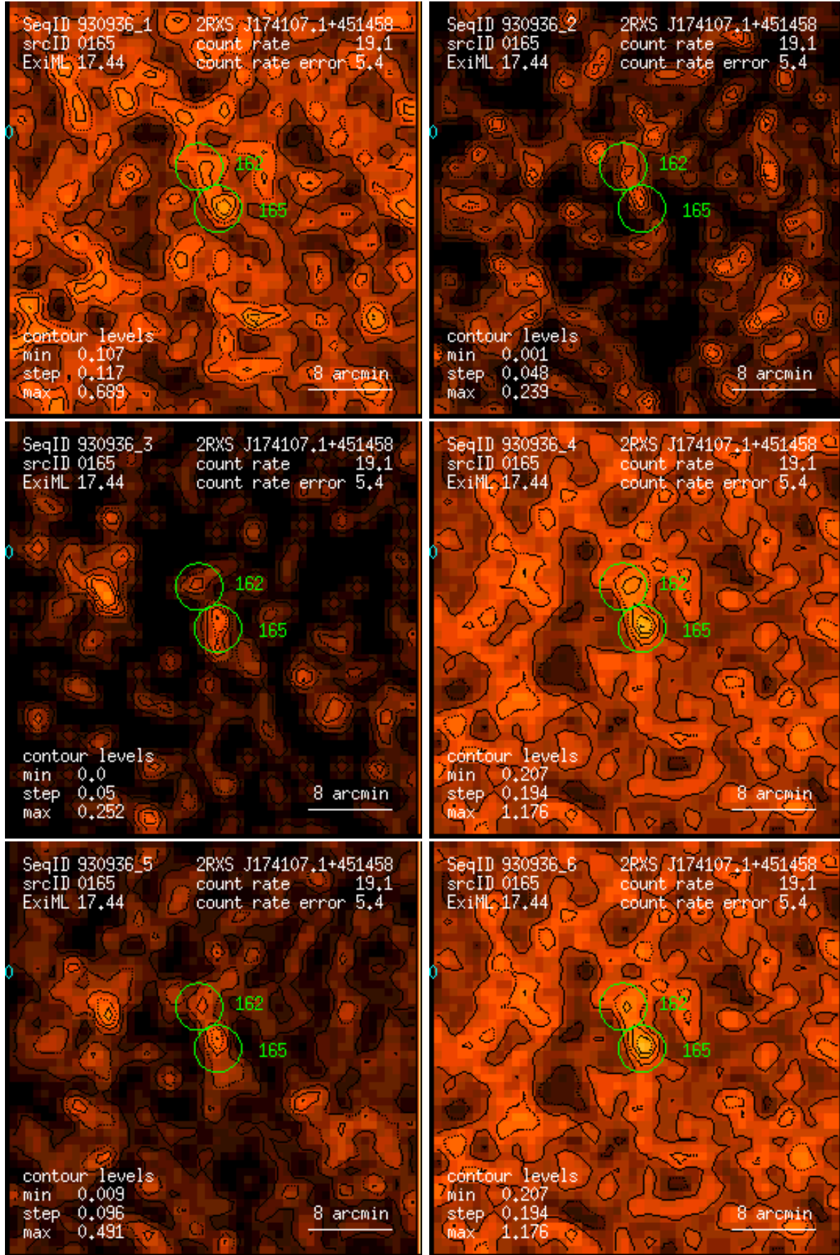
Figure 165: RASS 930936: detection 0165: band rate images, Gaussian filter: (1) PSPC channels 11 – 41, (2) 52 – 90, (3) 91 – 201, (4) 11 – 235, (5) 52 – 201, (6) 11 – 201. Broad band rates in counts/ks. Band rate contour levels in counts/ks/arcmin 2 .
