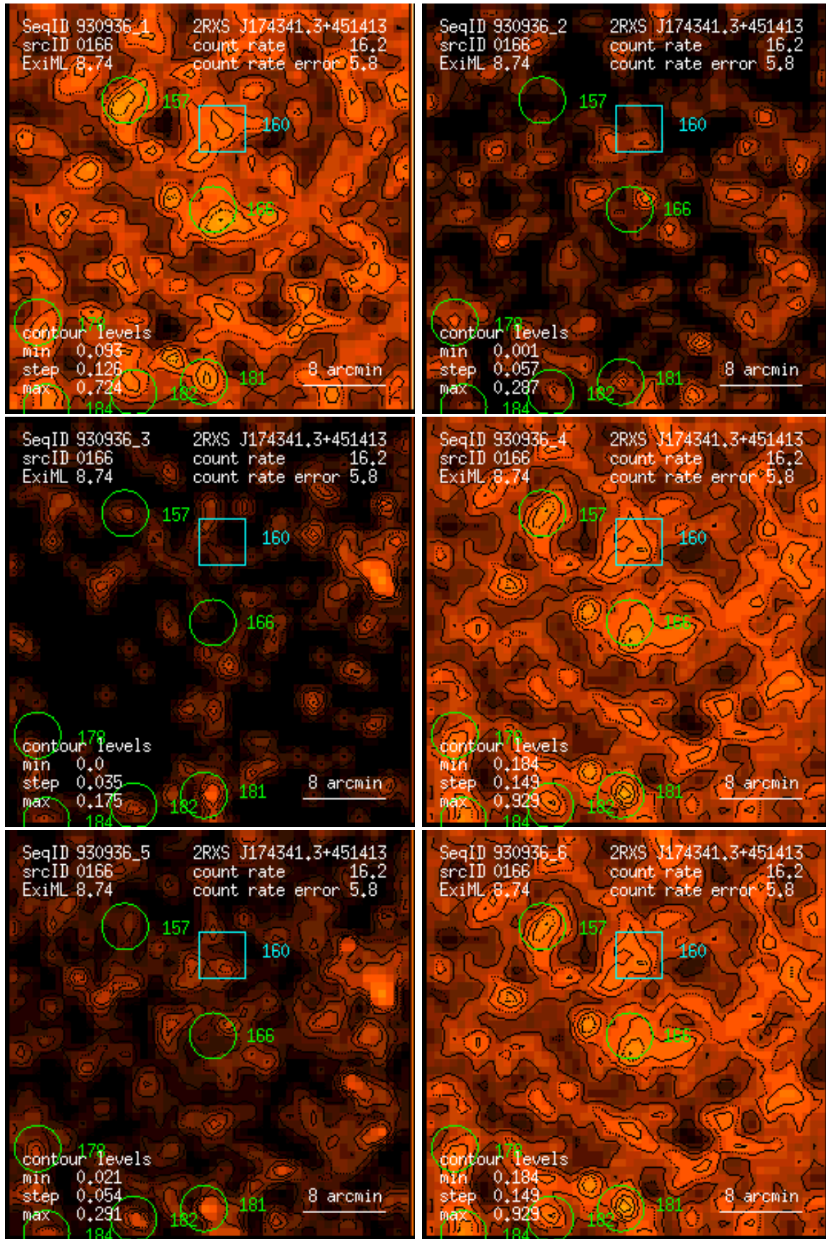
Figure 166: RASS 930936: detection 0166: band rate images, Gaussian filter: (1) PSPC channels 11 – 41, (2) 52 – 90, (3) 91 – 201, (4) 11 – 235, (5) 52 – 201, (6) 11 – 201. Broad band rates in counts/ks. Band rate contour levels in counts/ks/arcmin 2 .
