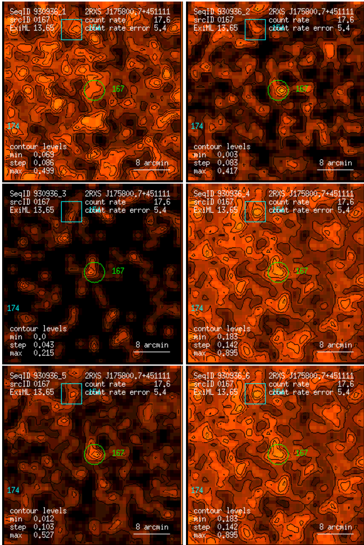
Figure 167: RASS 930936: detection 0167: band rate images, Gaussian filter: (1) PSPC channels 11 – 41, (2) 52 – 90, (3) 91 – 201, (4) 11 – 235, (5) 52 – 201, (6) 11 – 201. Broad band rates in counts/ks. Band rate contour levels in counts/ks/arcmin 2 .
