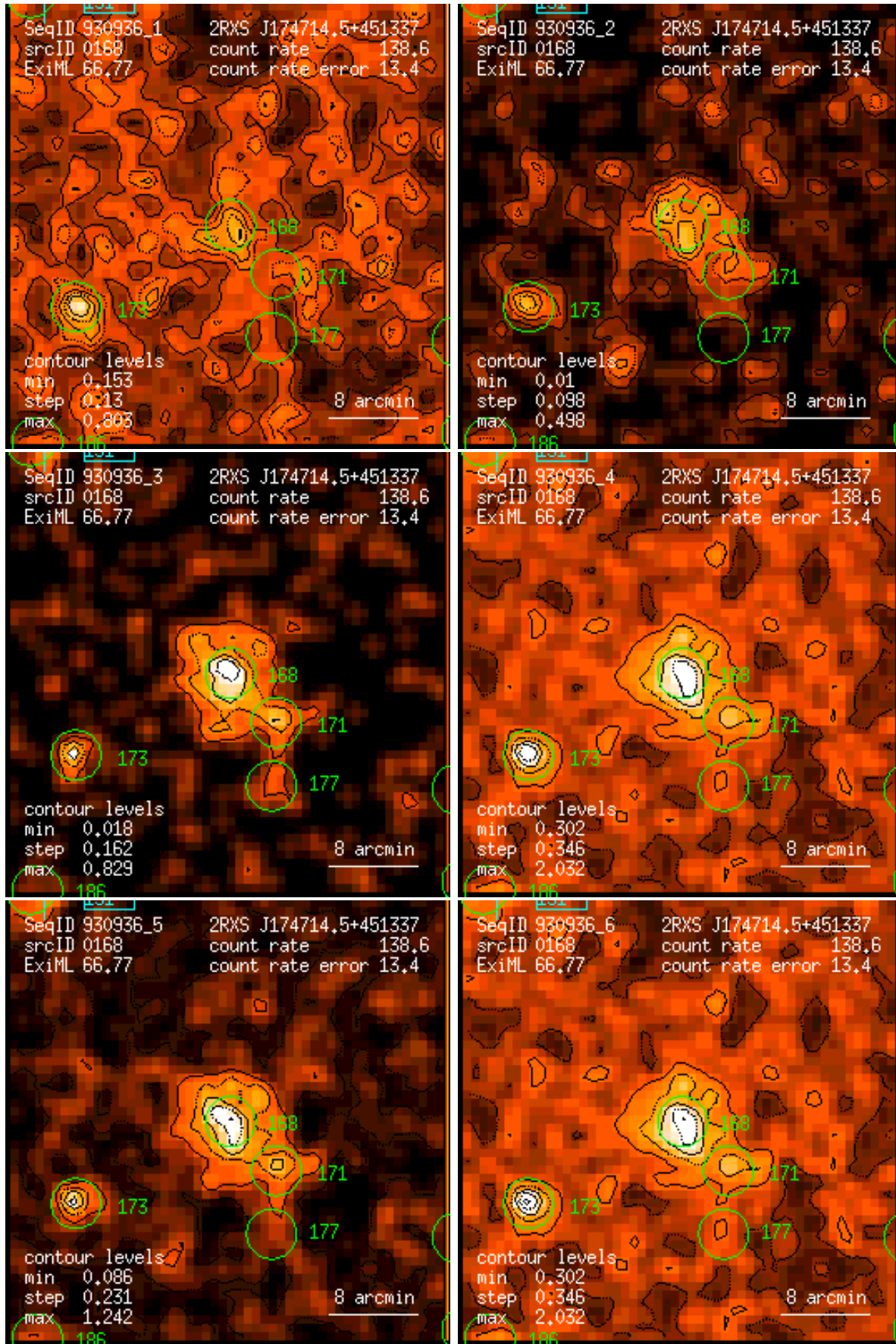
Figure 168: RASS 930936: detection 0168: band rate images, Gaussian filter: (1) PSPC channels 11 – 41, (2) 52 – 90, (3) 91 – 201, (4) 11 – 235, (5) 52 – 201, (6) 11 – 201. Broad band rates in counts/ks. Band rate contour levels in counts/ks/arcmin 2 .
