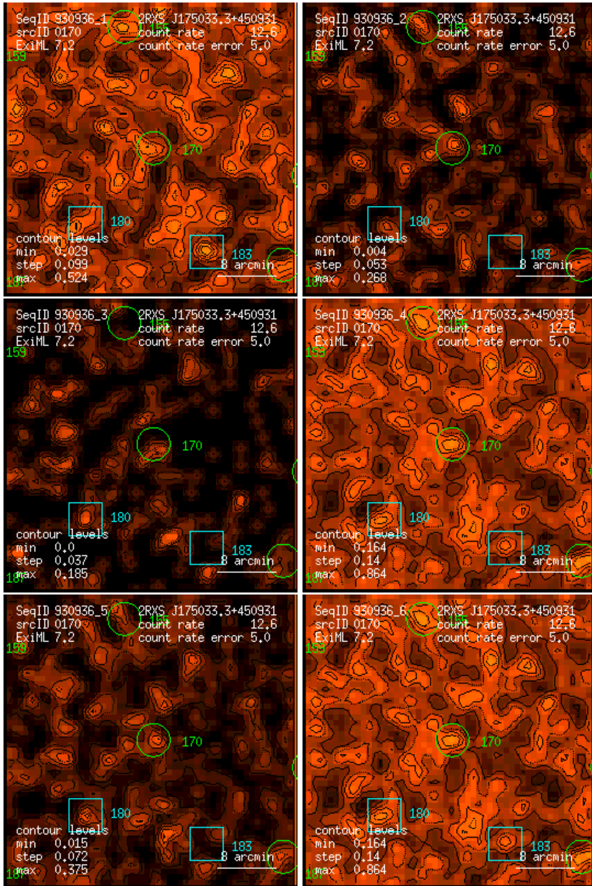
Figure 170: RASS 930936: detection 0170: band rate images, Gaussian filter: (1) PSPC channels 11 – 41, (2) 52 – 90, (3) 91 – 201, (4) 11 – 235, (5) 52 – 201, (6) 11 – 201. Broad band rates in counts/ks. Band rate contour levels in counts/ks/arcmin 2 .
