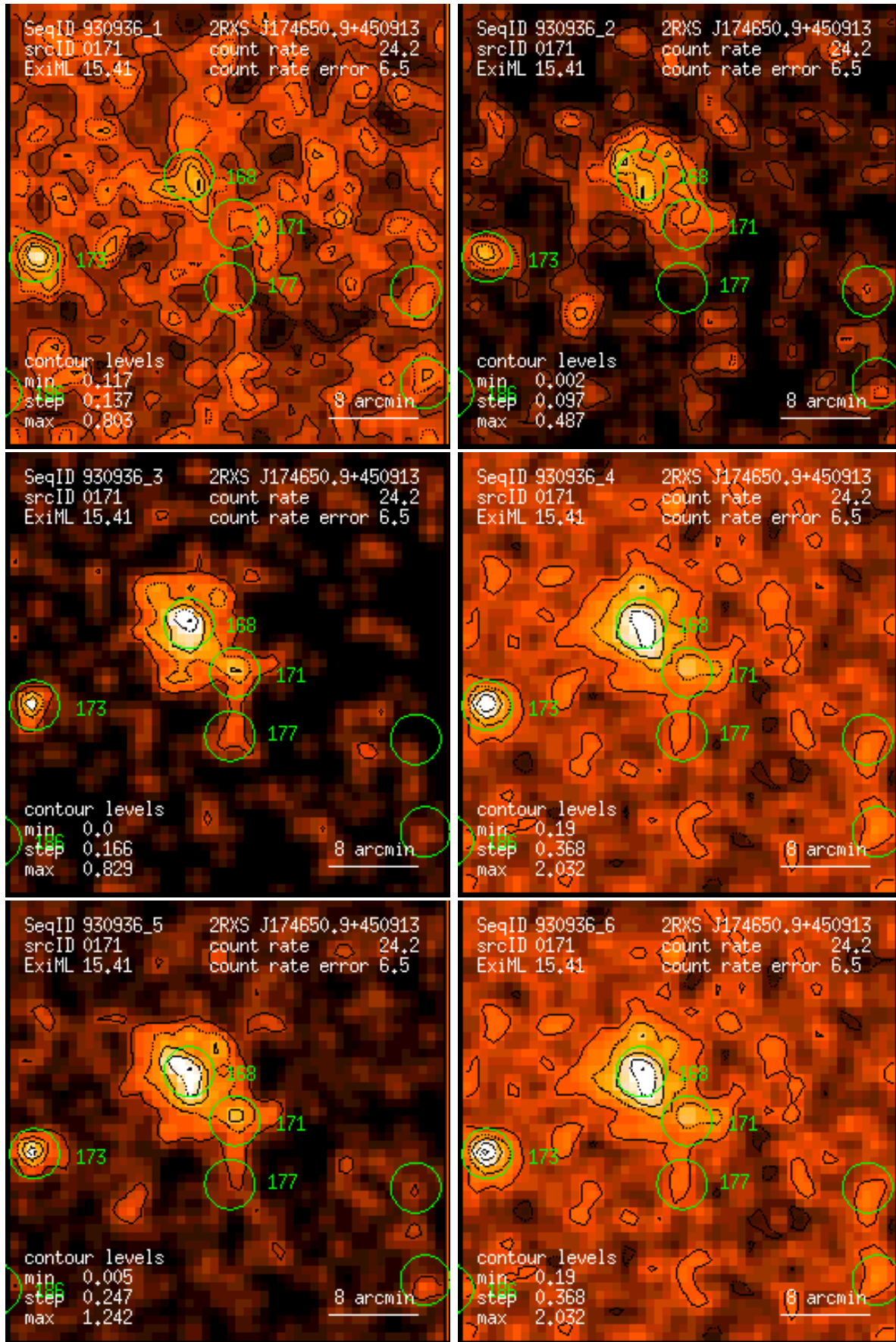
Figure 171: RASS 930936: detection 0171: band rate images, Gaussian filter: (1) PSPC channels 11 – 41, (2) 52 – 90, (3) 91 – 201, (4) 11 – 235, (5) 52 – 201, (6) 11 – 201. Broad band rates in counts/ks. Band rate contour levels in counts/ks/arcmin 2 .
