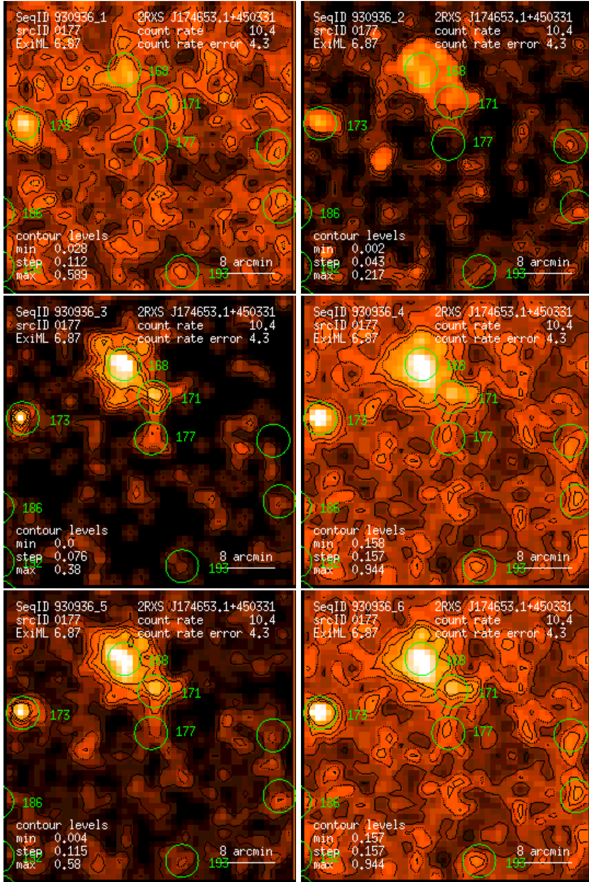
Figure 177: RASS 930936: detection 0177: band rate images, Gaussian filter: (1) PSPC channels 11 – 41, (2) 52 – 90, (3) 91 – 201, (4) 11 – 235, (5) 52 – 201, (6) 11 – 201. Broad band rates in counts/ks. Band rate contour levels in counts/ks/arcmin 2 .
