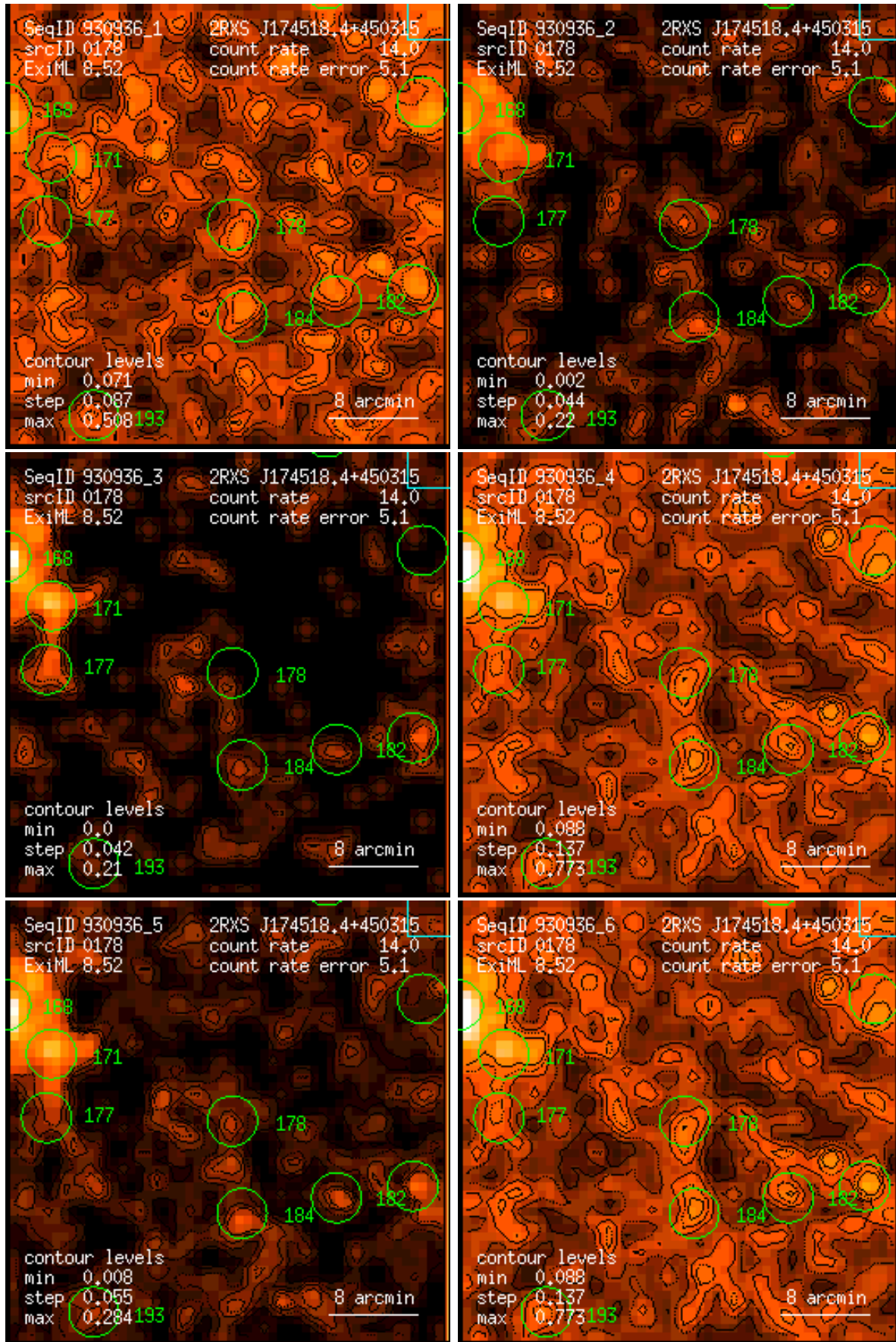
Figure 178: RASS 930936: detection 0178: band rate images, Gaussian filter: (1) PSPC channels 11 – 41, (2) 52 – 90, (3) 91 – 201, (4) 11 – 235, (5) 52 – 201, (6) 11 – 201. Broad band rates in counts/ks. Band rate contour levels in counts/ks/arcmin 2 .
