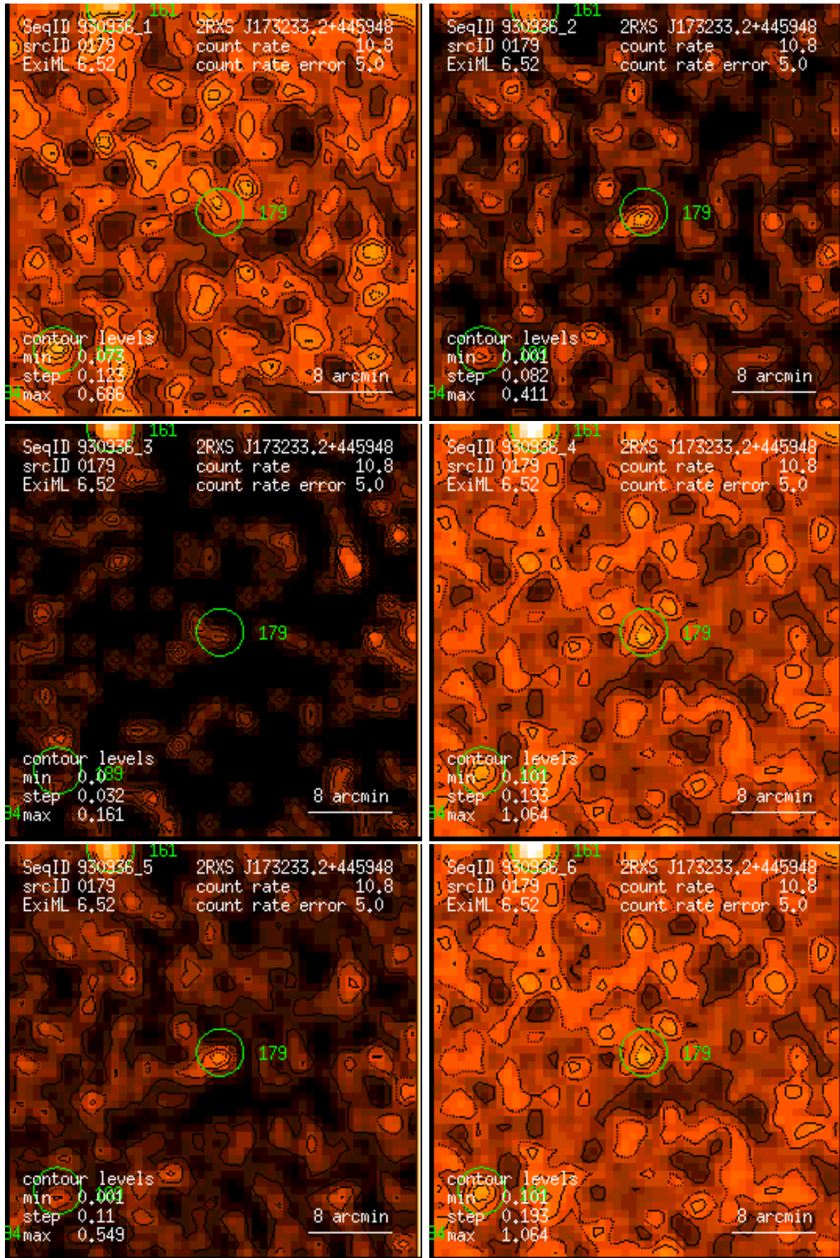
Figure 179: RASS 930936: detection 0179: band rate images, Gaussian filter: (1) PSPC channels 11 – 41, (2) 52 – 90, (3) 91 – 201, (4) 11 – 235, (5) 52 – 201, (6) 11 – 201. Broad band rates in counts/ks. Band rate contour levels in counts/ks/arcmin 2 .
