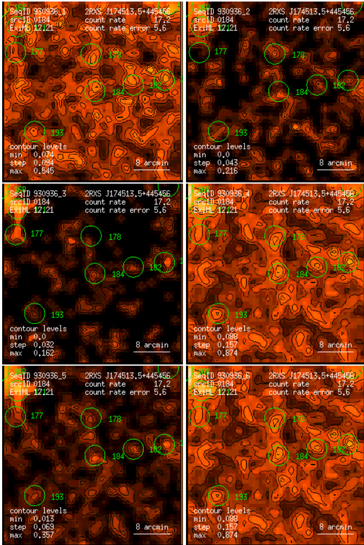
Figure 184: RASS 930936: detection 0184: band rate images, Gaussian filter: (1) PSPC channels 11 – 41, (2) 52 – 90, (3) 91 – 201, (4) 11 – 235, (5) 52 – 201, (6) 11 – 201. Broad band rates in counts/ks. Band rate contour levels in counts/ks/arcmin 2 .
