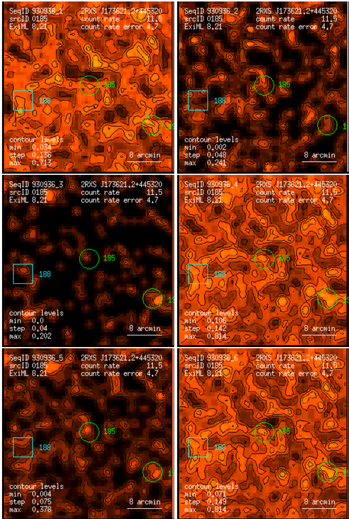
Figure 185: RASS 930936: detection 0185: band rate images, Gaussian filter: (1) PSPC channels 11 – 41, (2) 52 – 90, (3) 91 – 201, (4) 11 – 235, (5) 52 – 201, (6) 11 – 201. Broad band rates in counts/ks. Band rate contour levels in counts/ks/arcmin 2 .
