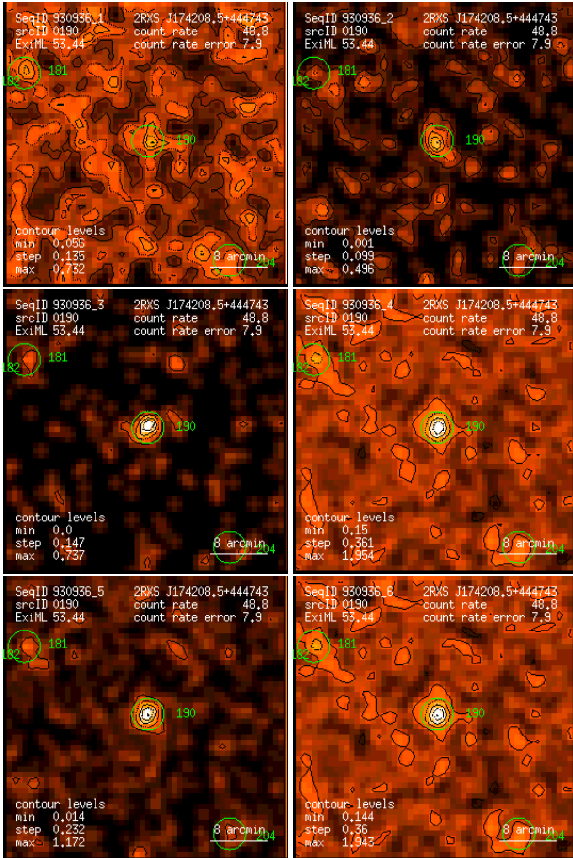
Figure 190: RASS 930936: detection 0190: band rate images, Gaussian filter: (1) PSPC channels 11 – 41, (2) 52 – 90, (3) 91 – 201, (4) 11 – 235, (5) 52 – 201, (6) 11 – 201. Broad band rates in counts/ks. Band rate contour levels in counts/ks/arcmin 2 .
