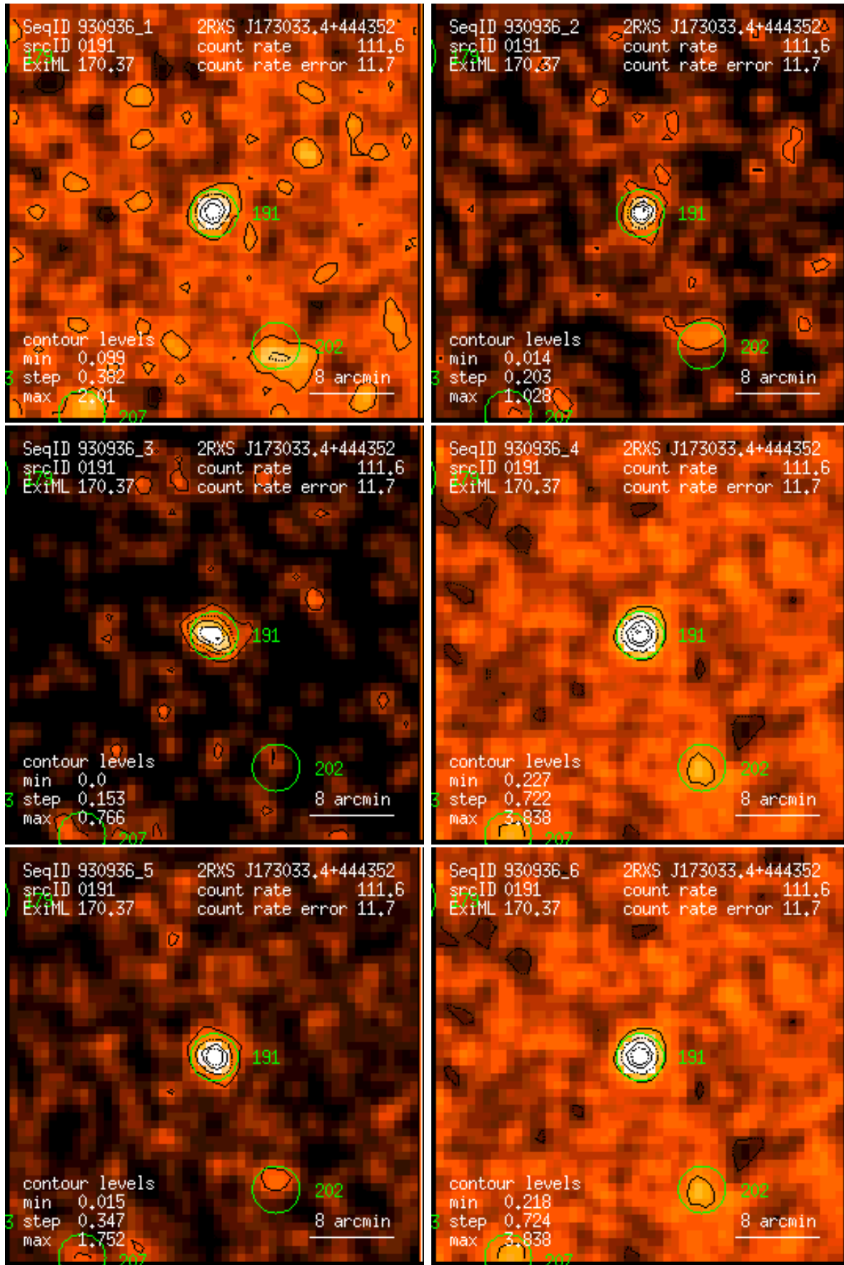
Figure 191: RASS 930936: detection 0191: band rate images, Gaussian filter: (1) PSPC channels 11 – 41, (2) 52 – 90, (3) 91 – 201, (4) 11 – 235, (5) 52 – 201, (6) 11 – 201. Broad band rates in counts/ks. Band rate contour levels in counts/ks/arcmin 2 .
