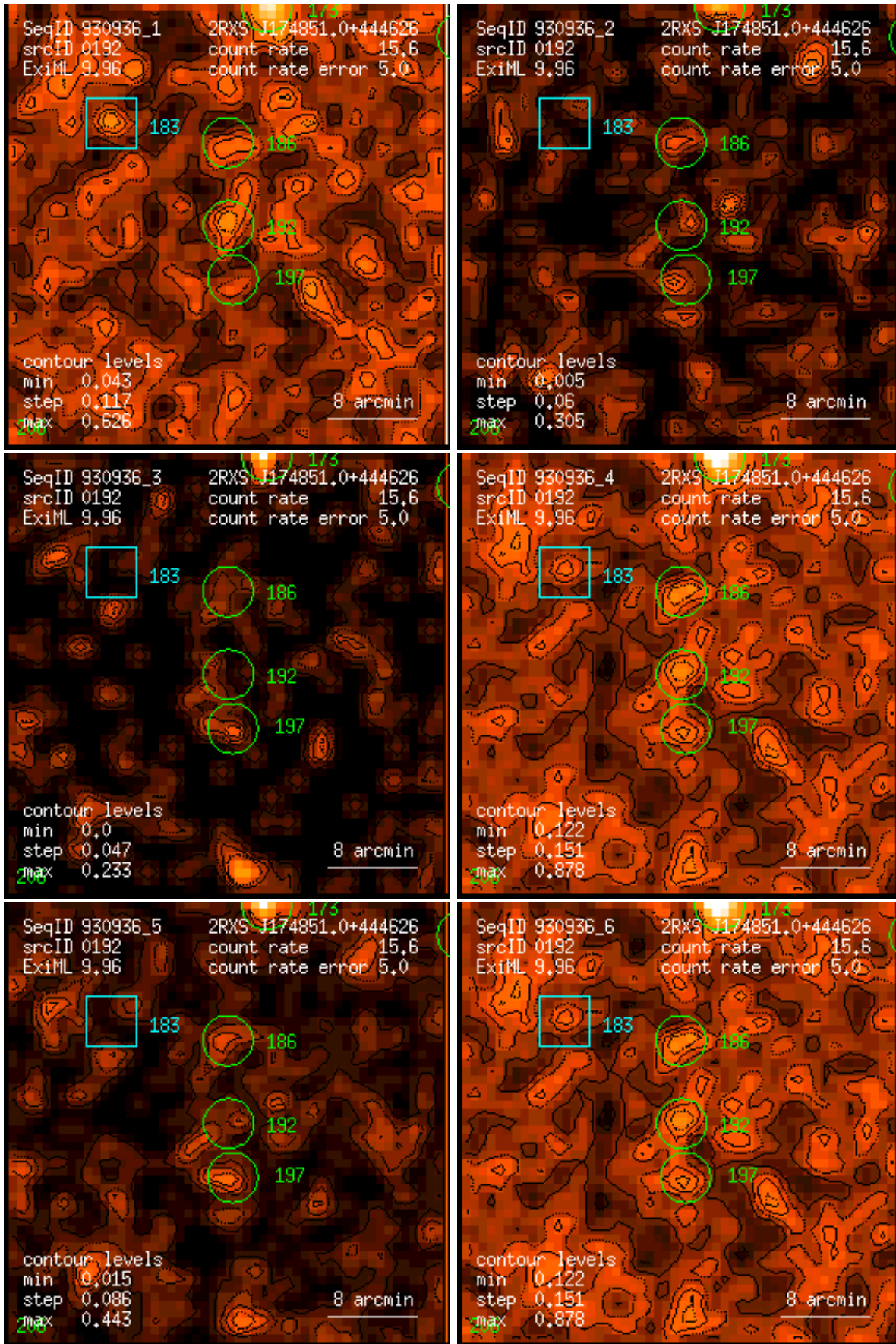
Figure 192: RASS 930936: detection 0192: band rate images, Gaussian filter: (1) PSPC channels 11 – 41, (2) 52 – 90, (3) 91 – 201, (4) 11 – 235, (5) 52 – 201, (6) 11 – 201. Broad band rates in counts/ks. Band rate contour levels in counts/ks/arcmin 2 .
