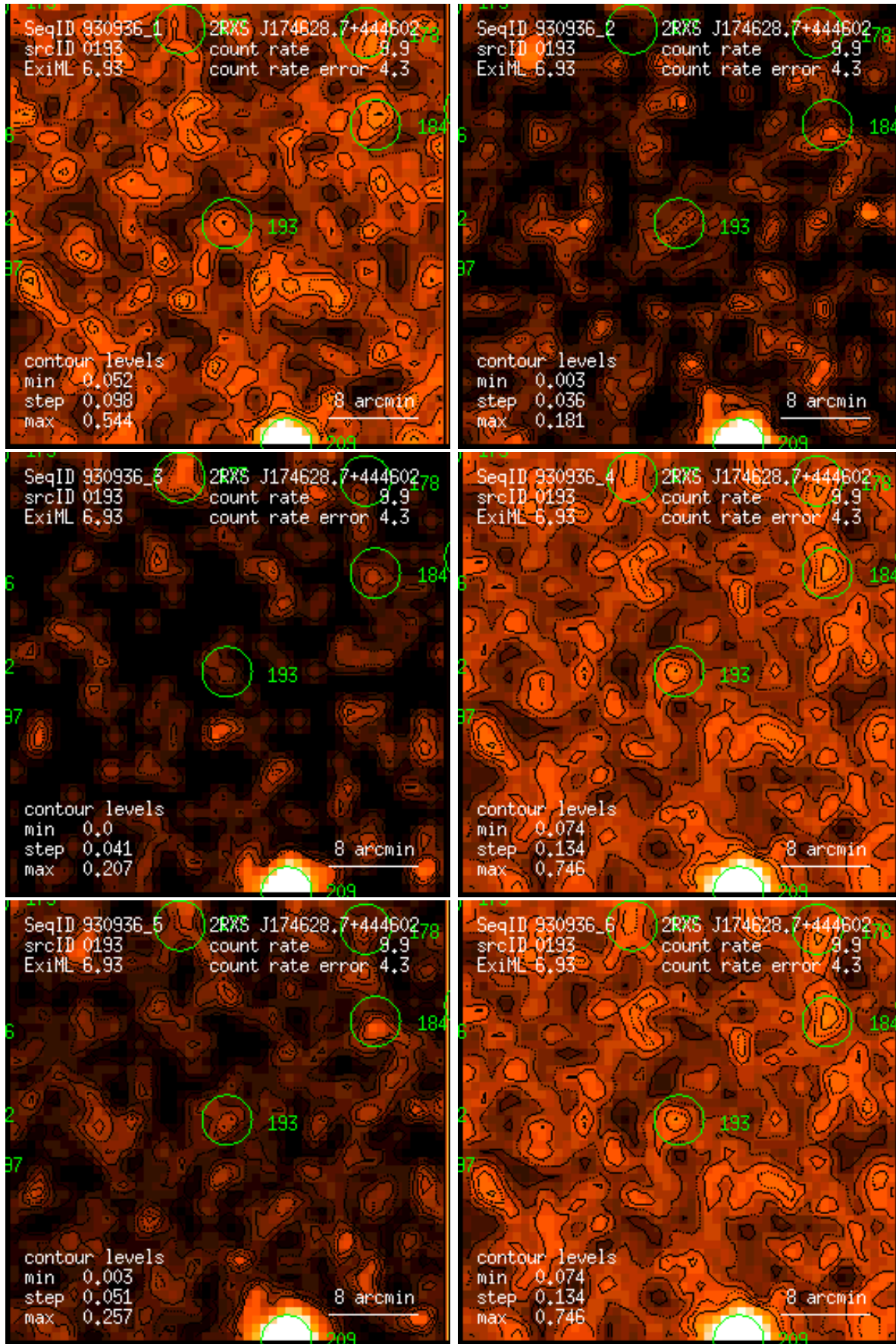
Figure 193: RASS 930936: detection 0193: band rate images, Gaussian filter: (1) PSPC channels 11 – 41, (2) 52 – 90, (3) 91 – 201, (4) 11 – 235, (5) 52 – 201, (6) 11 – 201. Broad band rates in counts/ks. Band rate contour levels in counts/ks/arcmin 2 .
