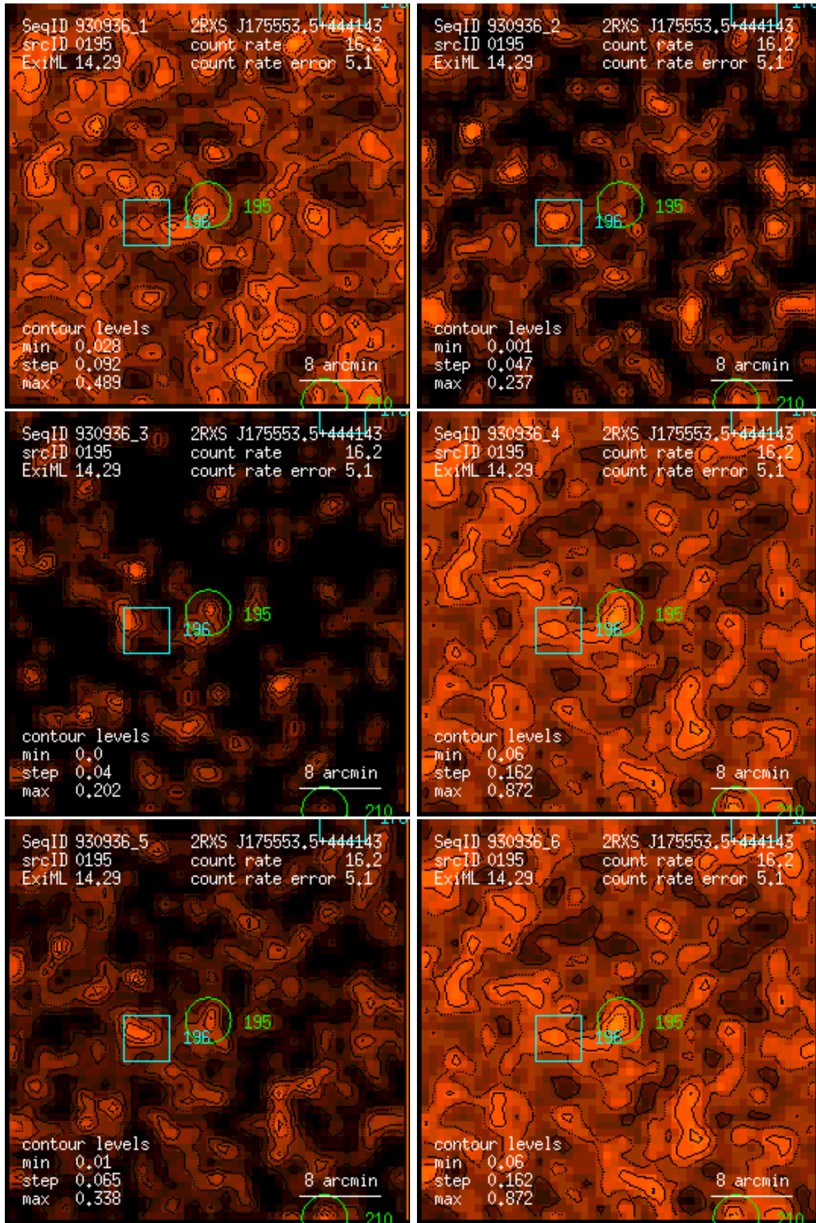
Figure 195: RASS 930936: detection 0195: band rate images, Gaussian filter: (1) PSPC channels 11 – 41, (2) 52 – 90, (3) 91 – 201, (4) 11 – 235, (5) 52 – 201, (6) 11 – 201. Broad band rates in counts/ks. Band rate contour levels in counts/ks/arcmin 2 .
