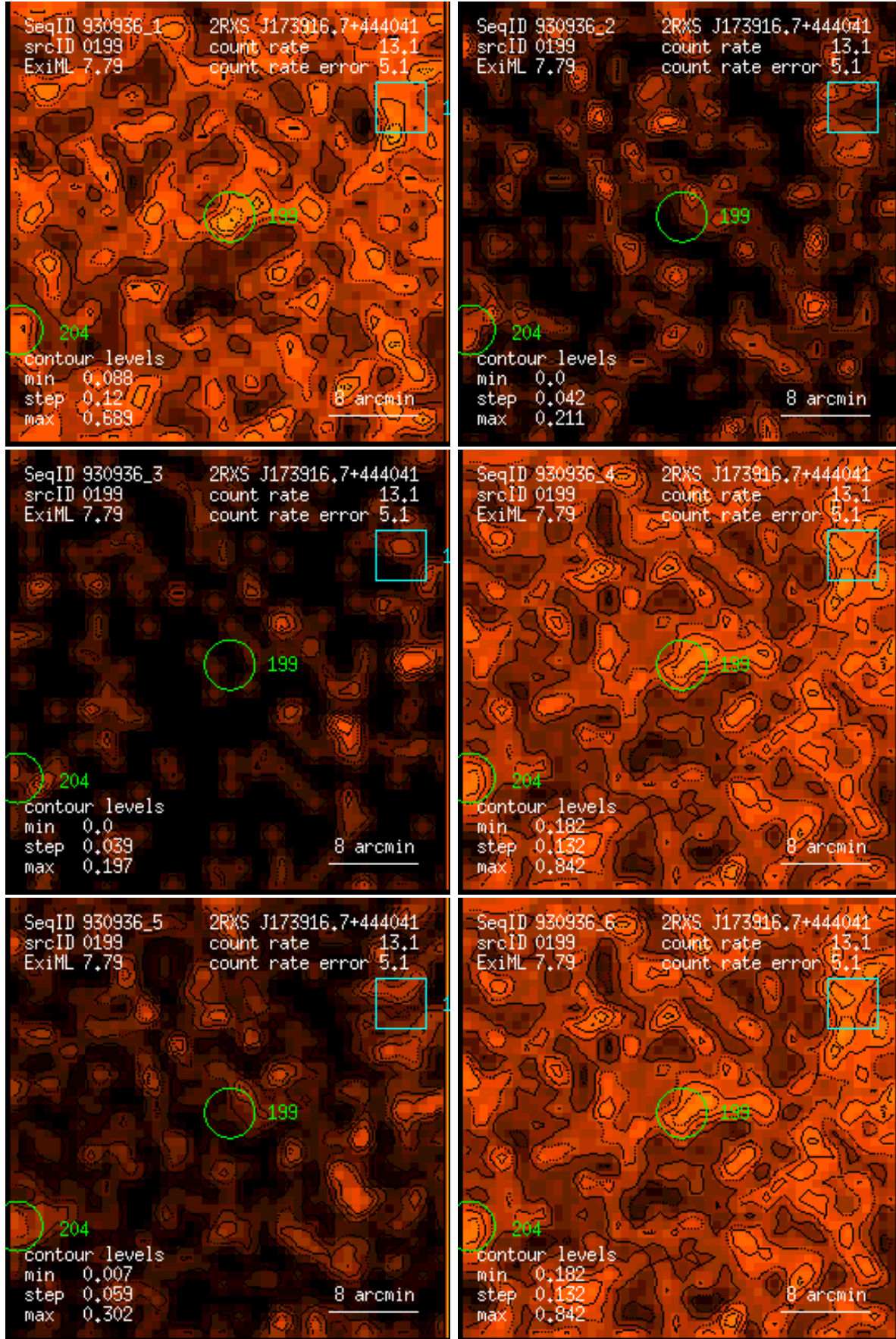
Figure 199: RASS 930936: detection 0199: band rate images, Gaussian filter: (1) PSPC channels 11 – 41, (2) 52 – 90, (3) 91 – 201, (4) 11 – 235, (5) 52 – 201, (6) 11 – 201. Broad band rates in counts/ks. Band rate contour levels in counts/ks/arcmin 2 .
