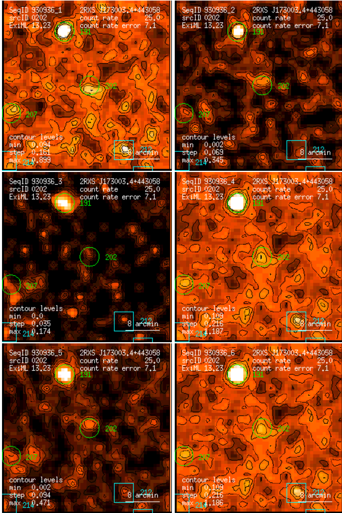
Figure 202: RASS 930936: detection 0202: band rate images, Gaussian filter: (1) PSPC channels 11 – 41, (2) 52 – 90, (3) 91 – 201, (4) 11 – 235, (5) 52 – 201, (6) 11 – 201. Broad band rates in counts/ks. Band rate contour levels in counts/ks/arcmin 2 .
