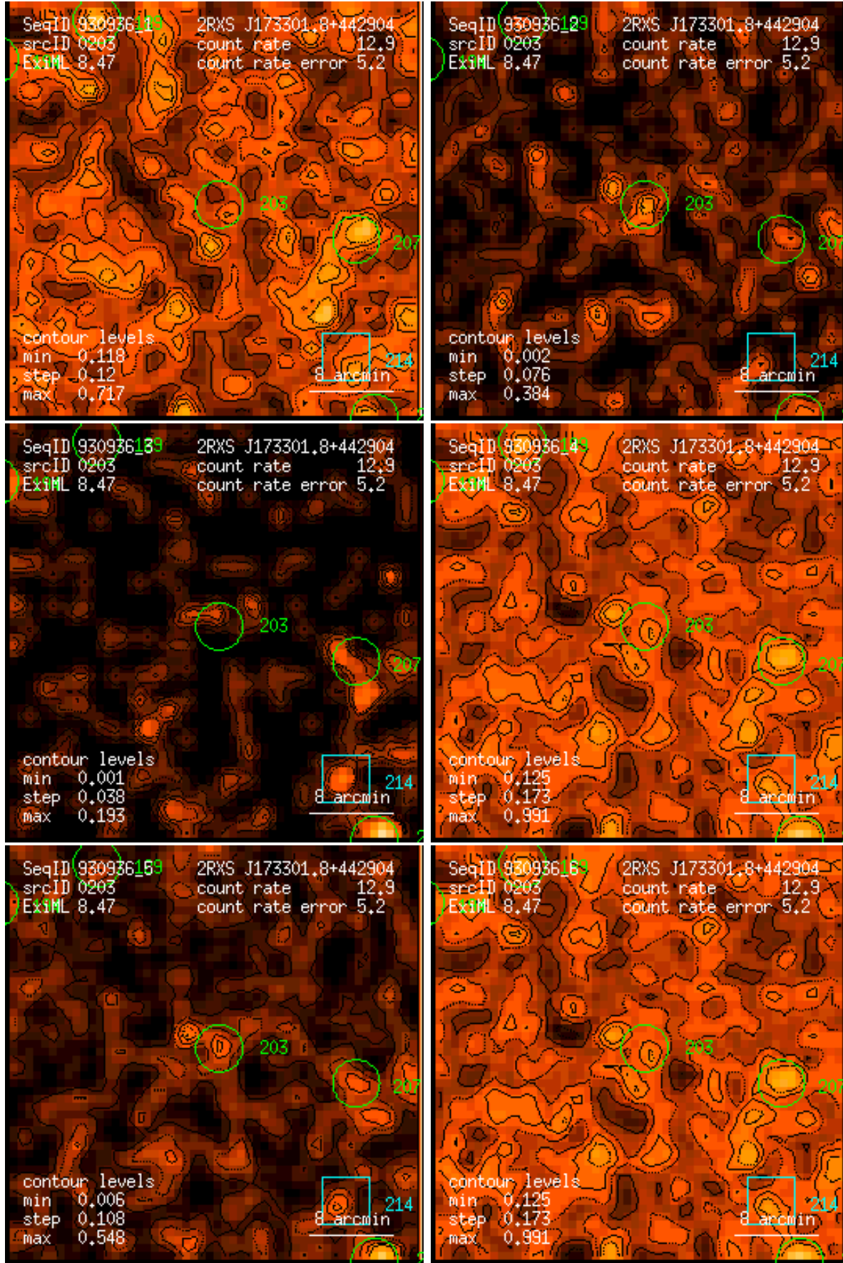
Figure 203: RASS 930936: detection 0203: band rate images, Gaussian filter: (1) PSPC channels 11 – 41, (2) 52 – 90, (3) 91 – 201, (4) 11 – 235, (5) 52 – 201, (6) 11 – 201. Broad band rates in counts/ks. Band rate contour levels in counts/ks/arcmin 2 .
