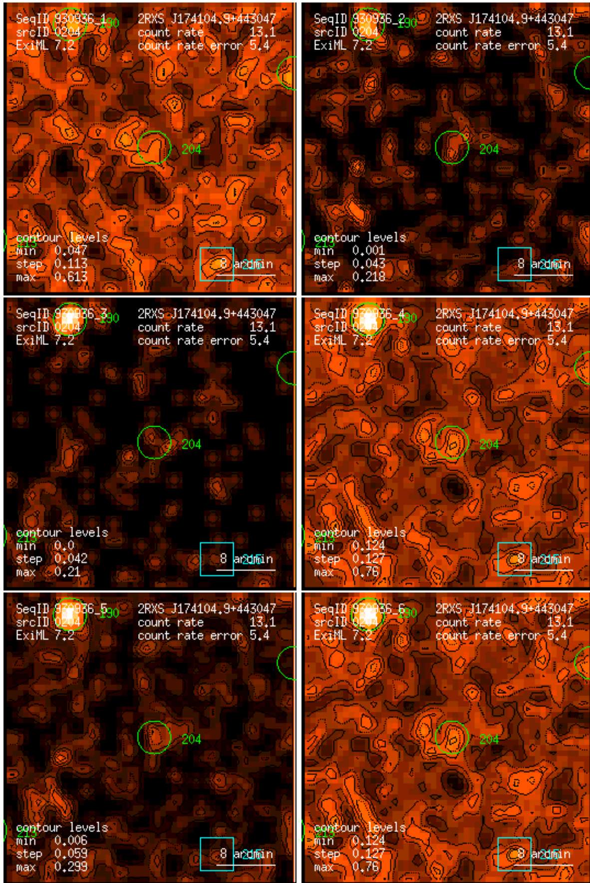
Figure 204: RASS 930936: detection 0204: band rate images, Gaussian filter: (1) PSPC channels 11 – 41, (2) 52 – 90, (3) 91 – 201, (4) 11 – 235, (5) 52 – 201, (6) 11 – 201. Broad band rates in counts/ks. Band rate contour levels in counts/ks/arcmin 2 .
