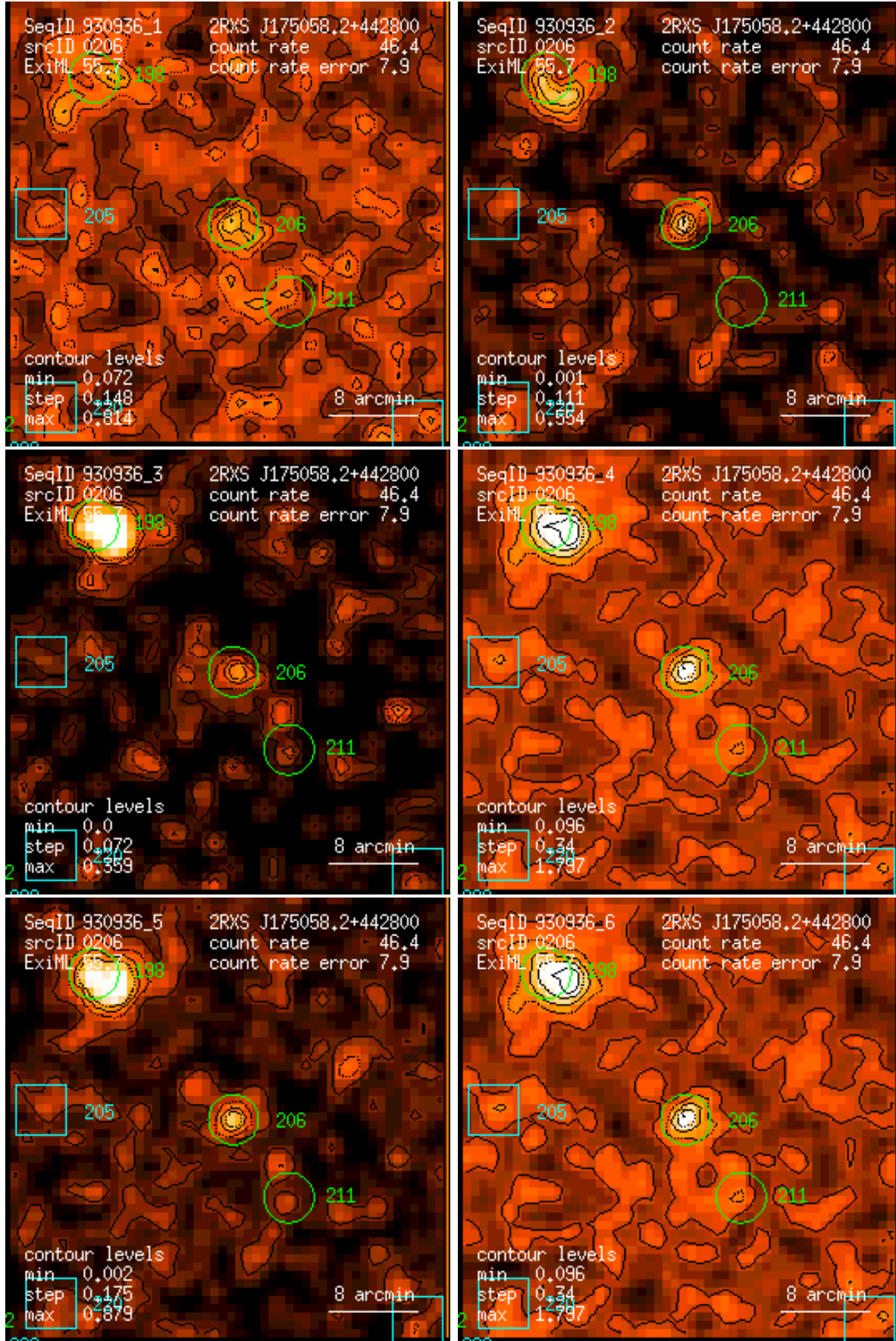
Figure 206: RASS 930936: detection 0206: band rate images, Gaussian filter: (1) PSPC channels 11 – 41, (2) 52 – 90, (3) 91 – 201, (4) 11 – 235, (5) 52 – 201, (6) 11 – 201. Broad band rates in counts/ks. Band rate contour levels in counts/ks/arcmin 2 .
