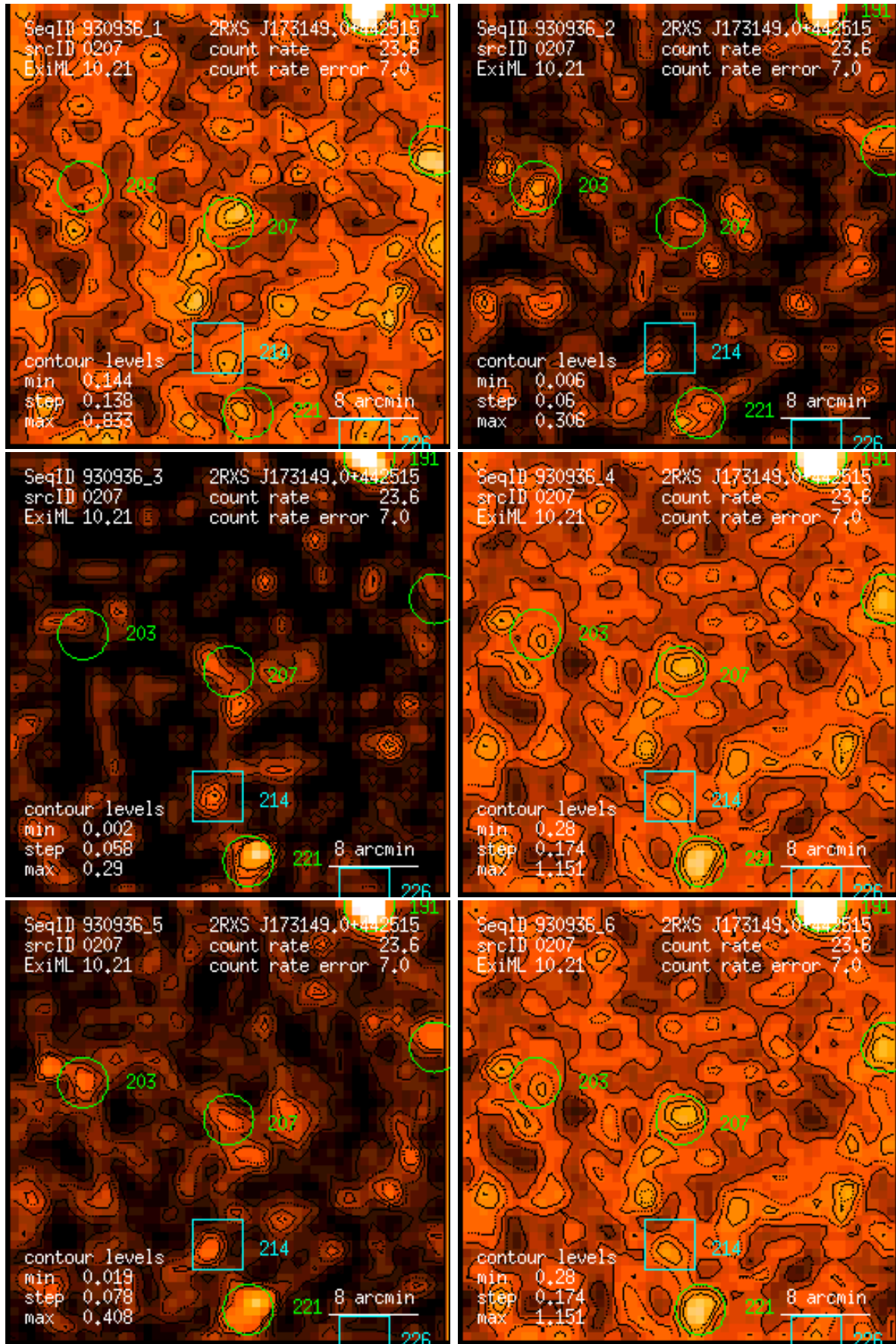
Figure 207: RASS 930936: detection 0207: band rate images, Gaussian filter: (1) PSPC channels 11 – 41, (2) 52 – 90, (3) 91 – 201, (4) 11 – 235, (5) 52 – 201, (6) 11 – 201. Broad band rates in counts/ks. Band rate contour levels in counts/ks/arcmin 2 .
