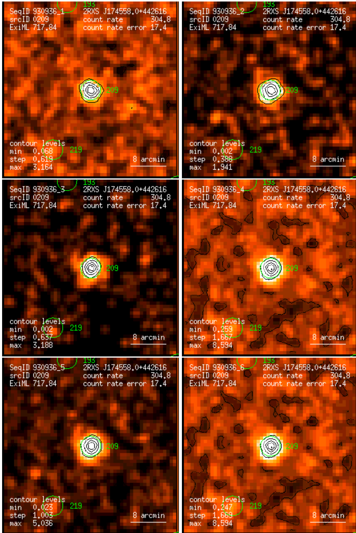
Figure 209: RASS 930936: detection 0209: band rate images, Gaussian filter: (1) PSPC channels 11 – 41, (2) 52 – 90, (3) 91 – 201, (4) 11 – 235, (5) 52 – 201, (6) 11 – 201. Broad band rates in counts/ks. Band rate contour levels in counts/ks/arcmin 2 .
