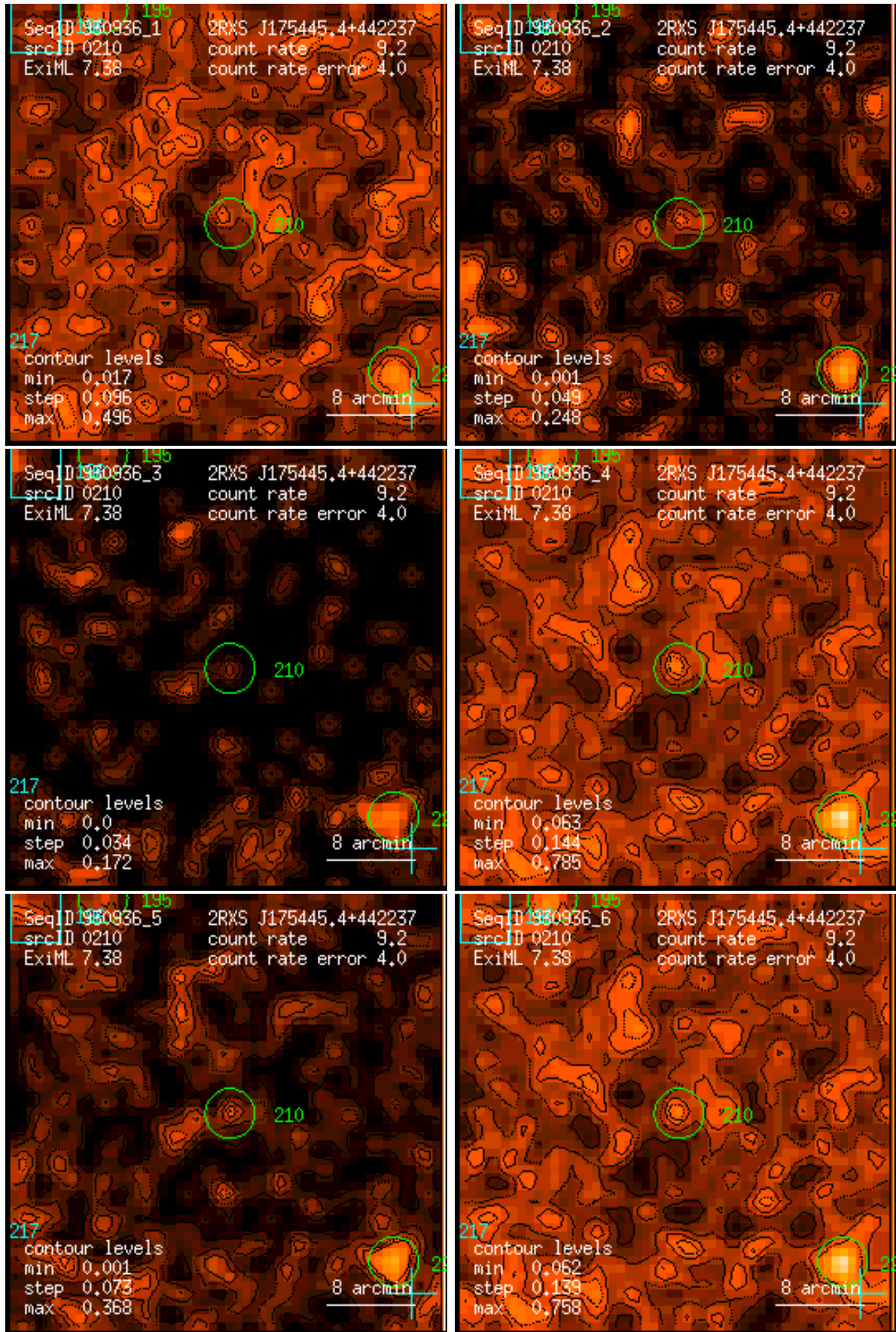
Figure 210: RASS 930936: detection 0210: band rate images, Gaussian filter: (1) PSPC channels 11 – 41, (2) 52 – 90, (3) 91 – 201, (4) 11 – 235, (5) 52 – 201, (6) 11 – 201. Broad band rates in counts/ks. Band rate contour levels in counts/ks/arcmin 2 .
