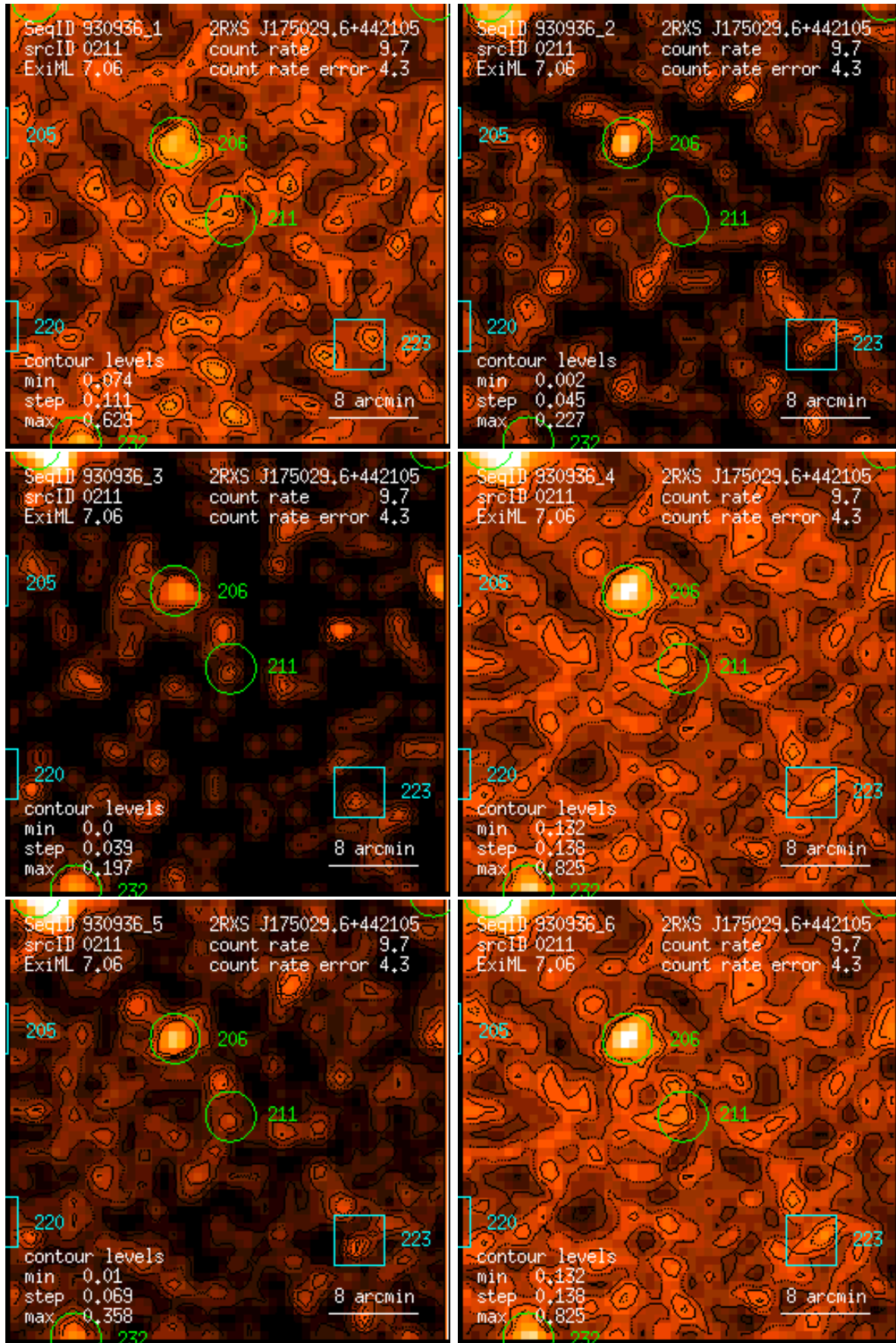
Figure 211: RASS 930936: detection 0211: band rate images, Gaussian filter: (1) PSPC channels 11 – 41, (2) 52 – 90, (3) 91 – 201, (4) 11 – 235, (5) 52 – 201, (6) 11 – 201. Broad band rates in counts/ks. Band rate contour levels in counts/ks/arcmin 2 .
