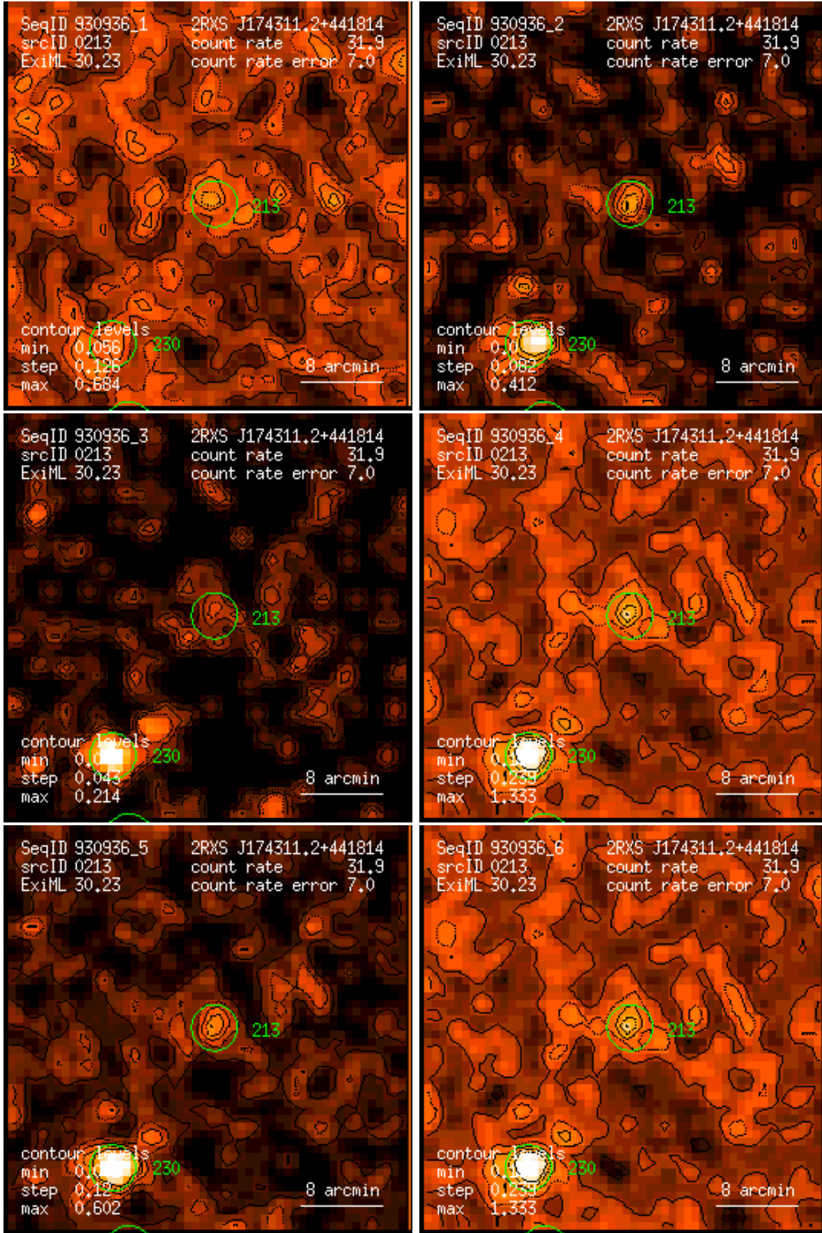
Figure 213: RASS 930936: detection 0213: band rate images, Gaussian filter: (1) PSPC channels 11 – 41, (2) 52 – 90, (3) 91 – 201, (4) 11 – 235, (5) 52 – 201, (6) 11 – 201. Broad band rates in counts/ks. Band rate contour levels in counts/ks/arcmin 2 .
