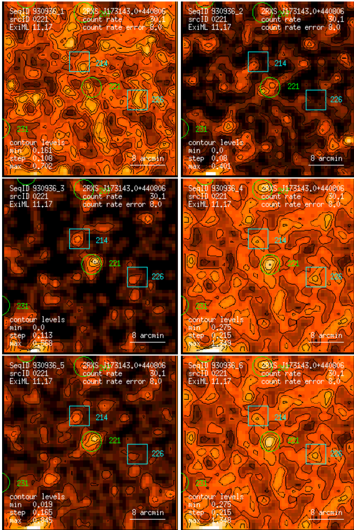
Figure 221: RASS 930936: detection 0221: band rate images, Gaussian filter: (1) PSPC channels 11 – 41, (2) 52 – 90, (3) 91 – 201, (4) 11 – 235, (5) 52 – 201, (6) 11 – 201. Broad band rates in counts/ks. Band rate contour levels in counts/ks/arcmin 2 .
