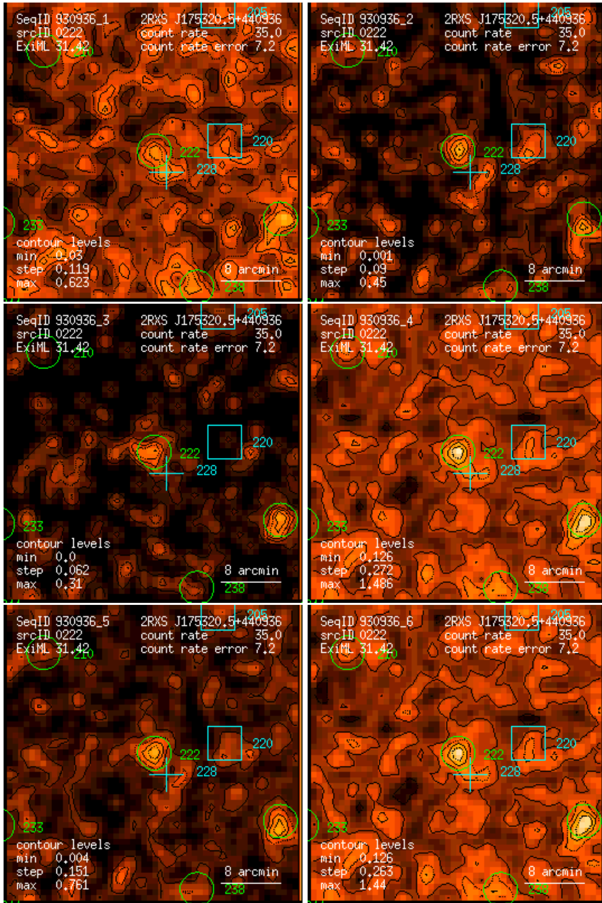
Figure 222: RASS 930936: detection 0222: band rate images, Gaussian filter: (1) PSPC channels 11 – 41, (2) 52 – 90, (3) 91 – 201, (4) 11 – 235, (5) 52 – 201, (6) 11 – 201. Broad band rates in counts/ks. Band rate contour levels in counts/ks/arcmin 2 .
