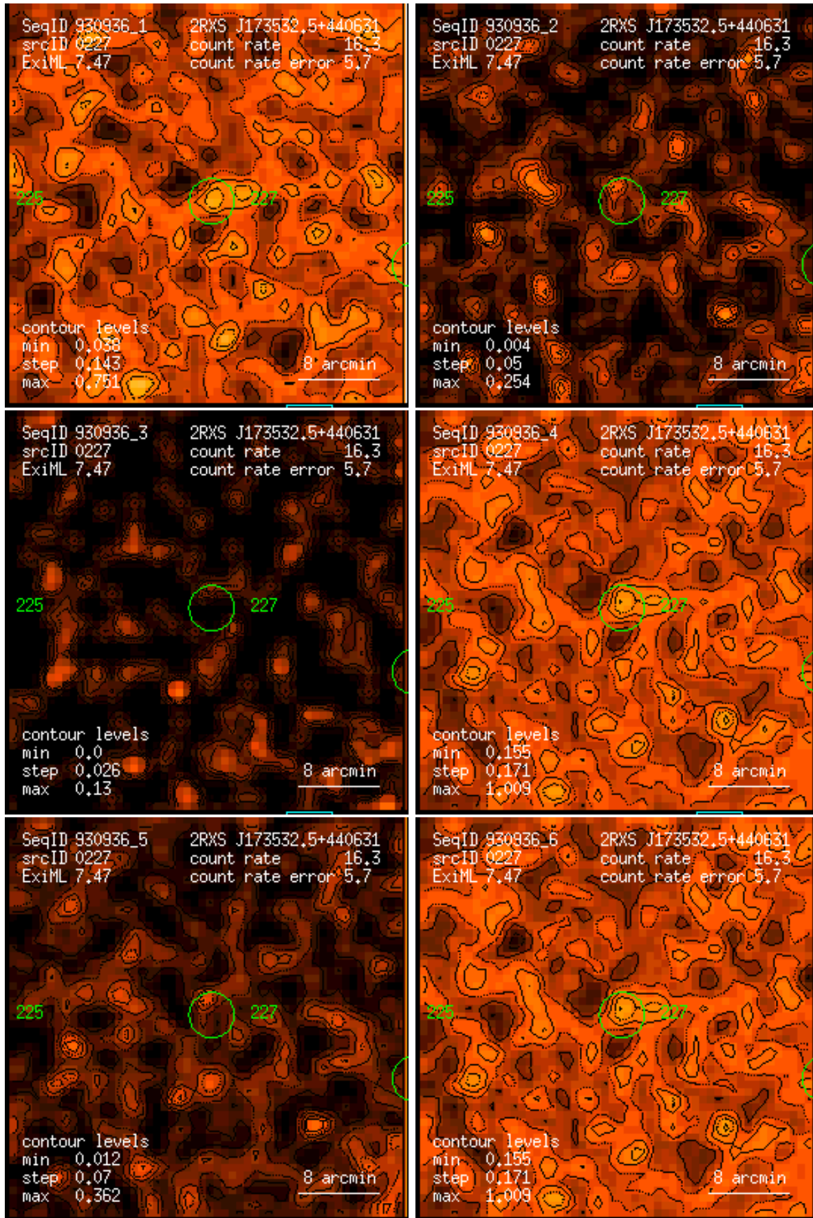
Figure 227: RASS 930936: detection 0227: band rate images, Gaussian filter: (1) PSPC channels 11 – 41, (2) 52 – 90, (3) 91 – 201, (4) 11 – 235, (5) 52 – 201, (6) 11 – 201. Broad band rates in counts/ks. Band rate contour levels in counts/ks/arcmin 2 .
