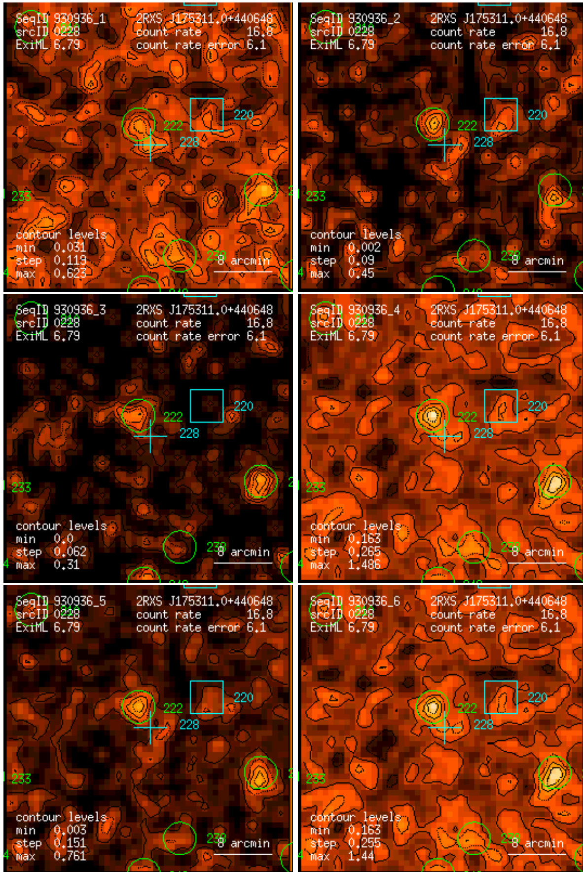
Figure 228: RASS 930936: detection 0228: band rate images, Gaussian filter: (1) PSPC channels 11 – 41, (2) 52 – 90, (3) 91 – 201, (4) 11 – 235, (5) 52 – 201, (6) 11 – 201. Broad band rates in counts/ks. Band rate contour levels in counts/ks/arcmin 2 .
