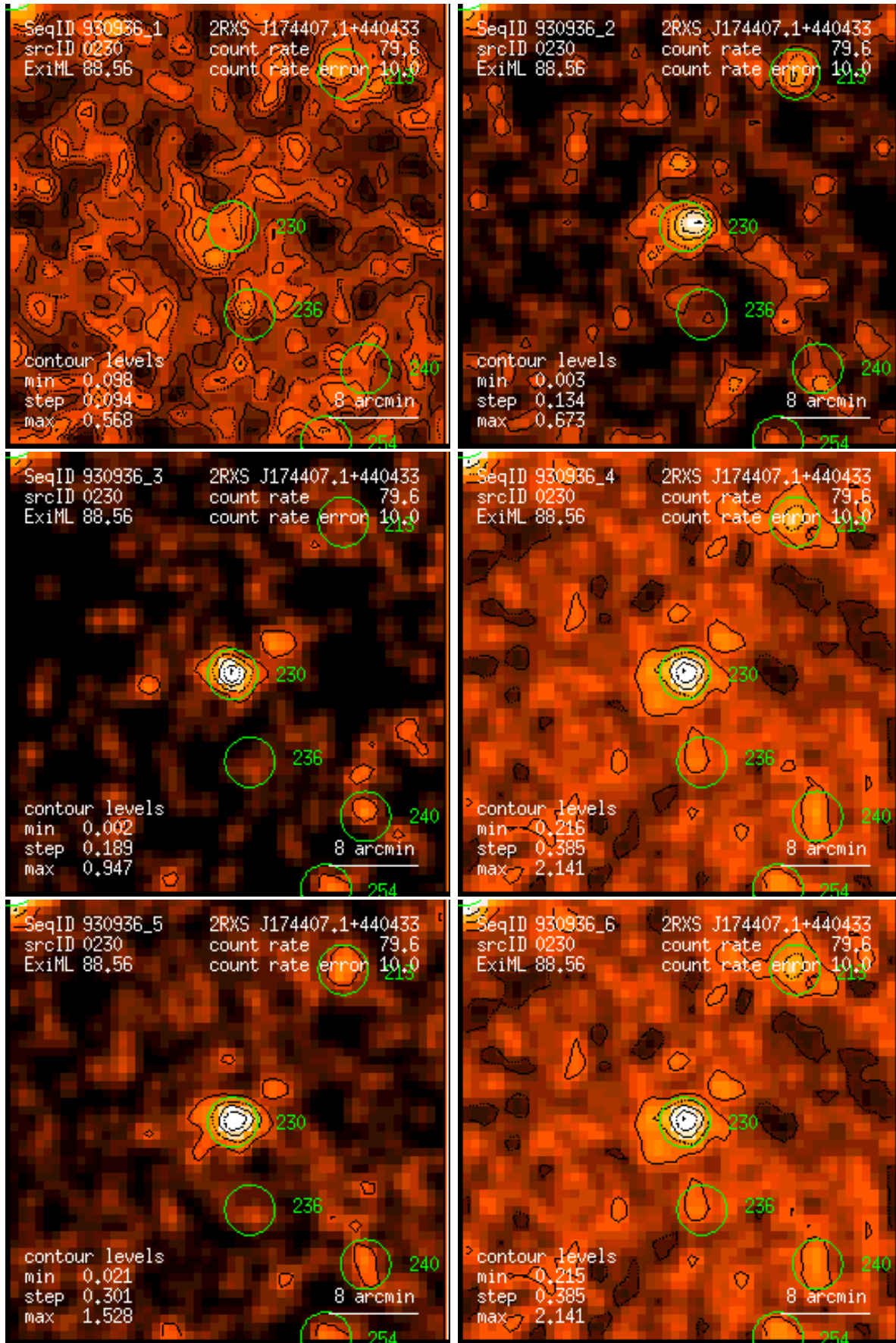
Figure 230: RASS 930936: detection 0230: band rate images, Gaussian filter: (1) PSPC channels 11 – 41, (2) 52 – 90, (3) 91 – 201, (4) 11 – 235, (5) 52 – 201, (6) 11 – 201. Broad band rates in counts/ks. Band rate contour levels in counts/ks/arcmin 2 .
