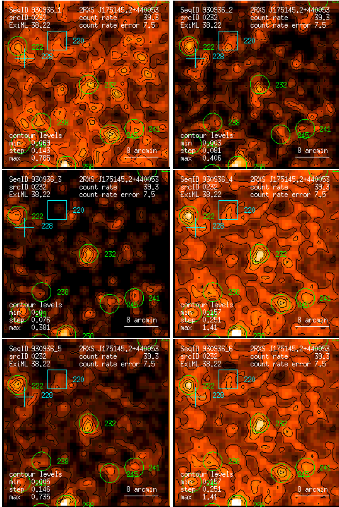
Figure 232: RASS 930936: detection 0232: band rate images, Gaussian filter: (1) PSPC channels 11 – 41, (2) 52 – 90, (3) 91 – 201, (4) 11 – 235, (5) 52 – 201, (6) 11 – 201. Broad band rates in counts/ks. Band rate contour levels in counts/ks/arcmin 2 .
