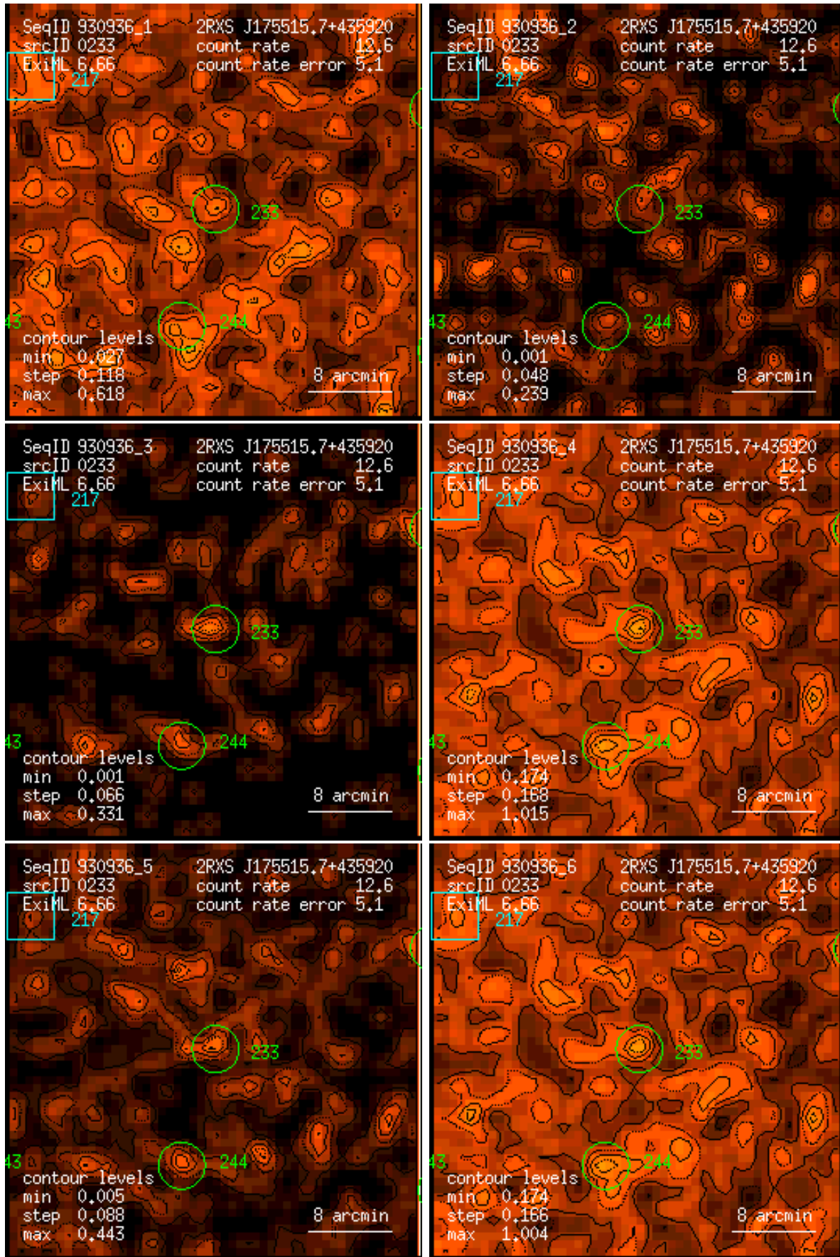
Figure 233: RASS 930936: detection 0233: band rate images, Gaussian filter: (1) PSPC channels 11 – 41, (2) 52 – 90, (3) 91 – 201, (4) 11 – 235, (5) 52 – 201, (6) 11 – 201. Broad band rates in counts/ks. Band rate contour levels in counts/ks/arcmin 2 .
