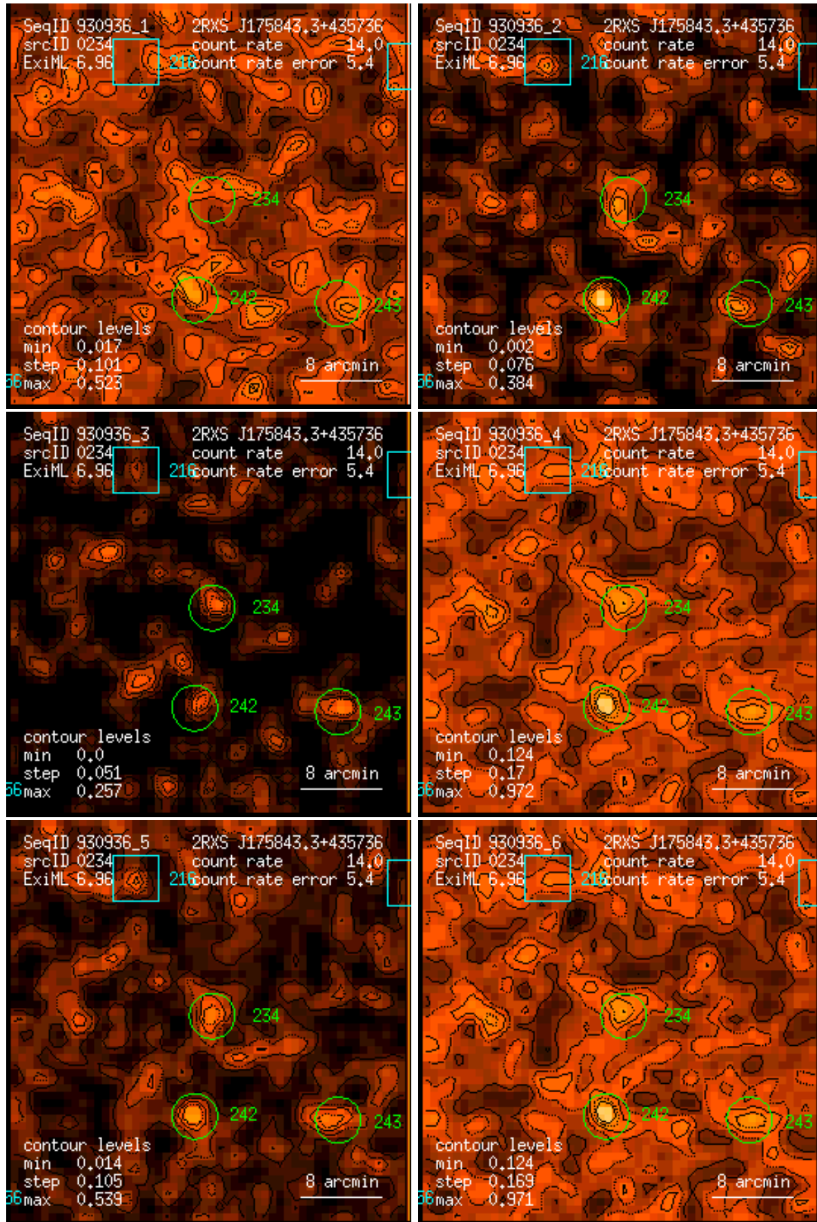
Figure 234: RASS 930936: detection 0234: band rate images, Gaussian filter: (1) PSPC channels 11 – 41, (2) 52 – 90, (3) 91 – 201, (4) 11 – 235, (5) 52 – 201, (6) 11 – 201. Broad band rates in counts/ks. Band rate contour levels in counts/ks/arcmin 2 .
