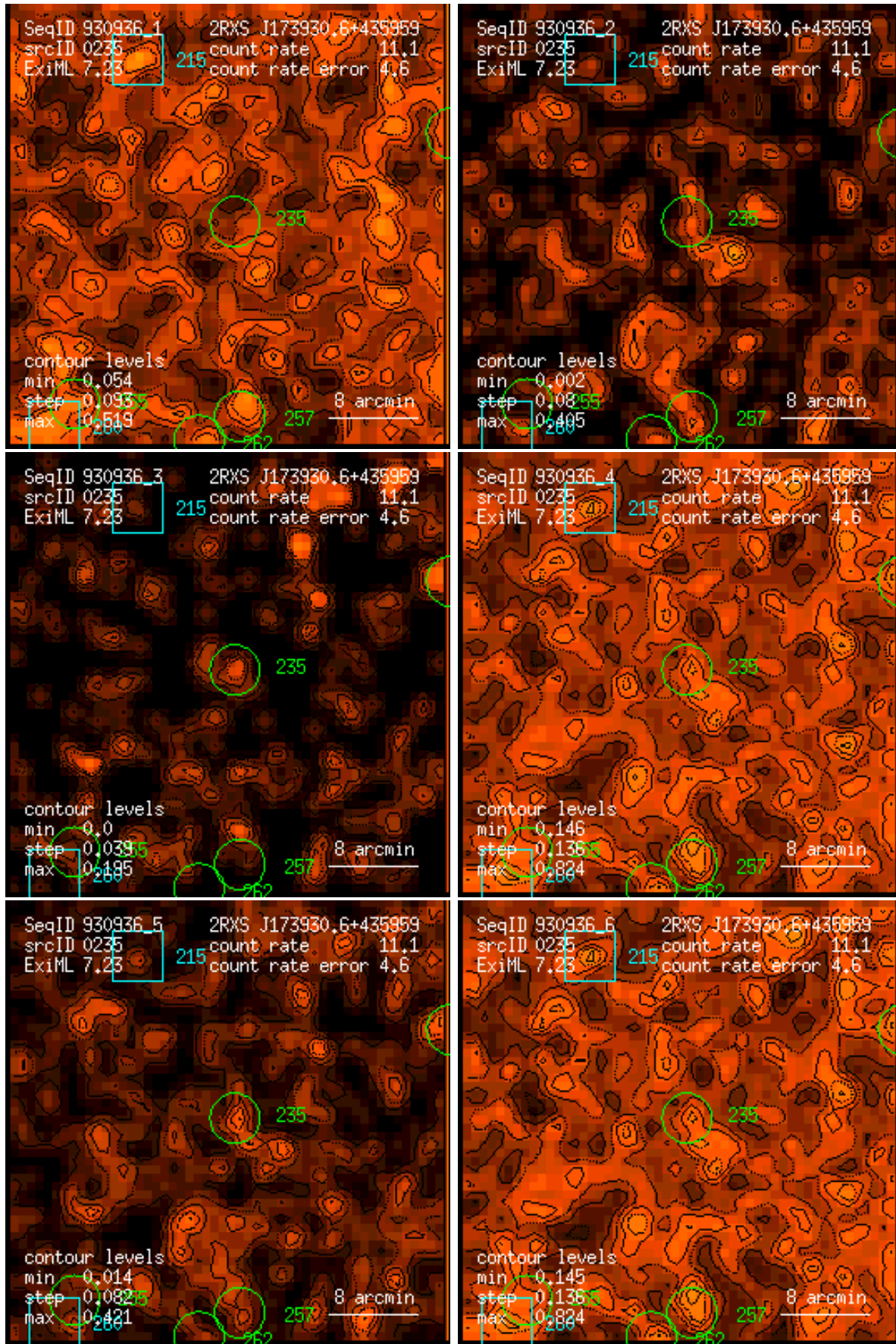
Figure 235: RASS 930936: detection 0235: band rate images, Gaussian filter: (1) PSPC channels 11 – 41, (2) 52 – 90, (3) 91 – 201, (4) 11 – 235, (5) 52 – 201, (6) 11 – 201. Broad band rates in counts/ks. Band rate contour levels in counts/ks/arcmin 2 .
