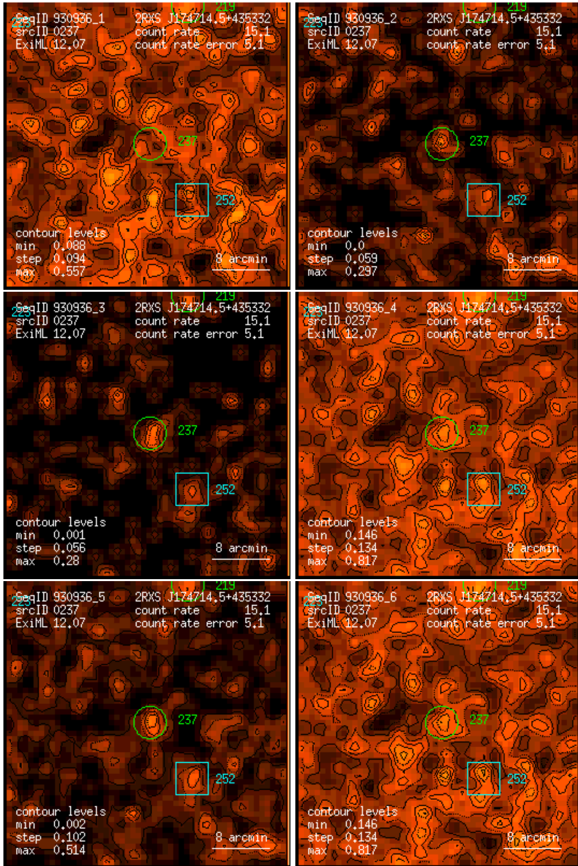
Figure 237: RASS 930936: detection 0237: band rate images, Gaussian filter: (1) PSPC channels 11 – 41, (2) 52 – 90, (3) 91 – 201, (4) 11 – 235, (5) 52 – 201, (6) 11 – 201. Broad band rates in counts/ks. Band rate contour levels in counts/ks/arcmin 2 .
