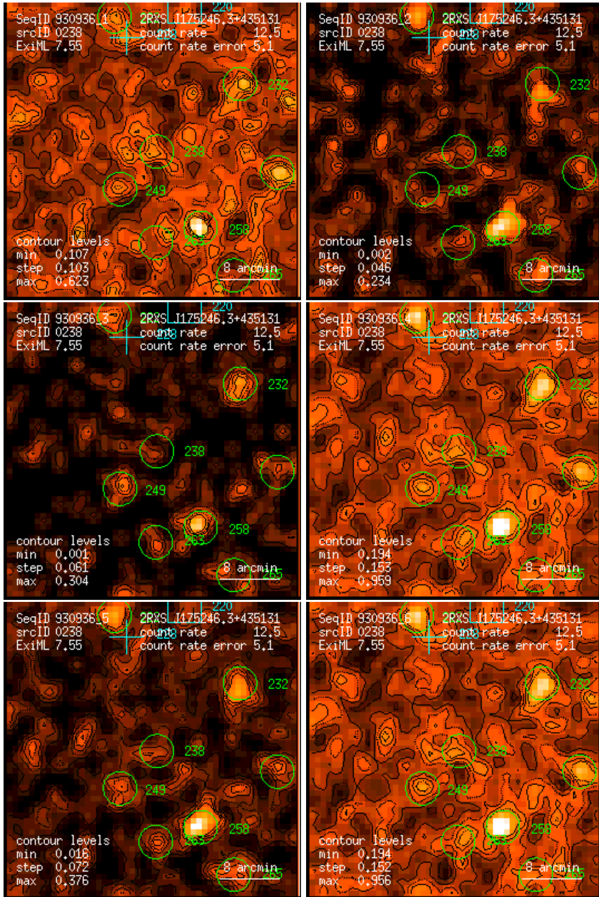
Figure 238: RASS 930936: detection 0238: band rate images, Gaussian filter: (1) PSPC channels 11 – 41, (2) 52 – 90, (3) 91 – 201, (4) 11 – 235, (5) 52 – 201, (6) 11 – 201. Broad band rates in counts/ks. Band rate contour levels in counts/ks/arcmin 2 .
