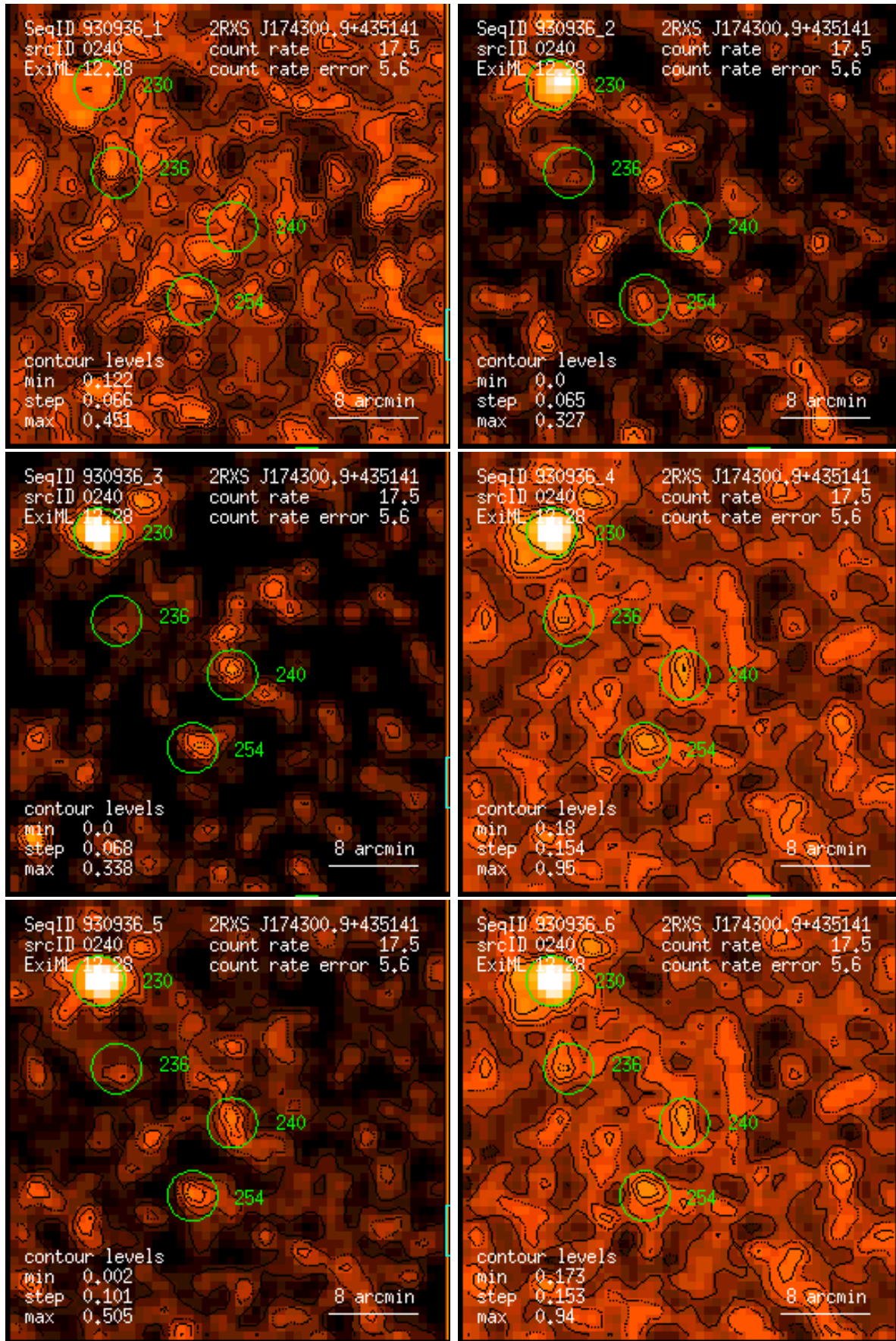
Figure 240: RASS 930936: detection 0240: band rate images, Gaussian filter: (1) PSPC channels 11 – 41, (2) 52 – 90, (3) 91 – 201, (4) 11 – 235, (5) 52 – 201, (6) 11 – 201. Broad band rates in counts/ks. Band rate contour levels in counts/ks/arcmin 2 .
