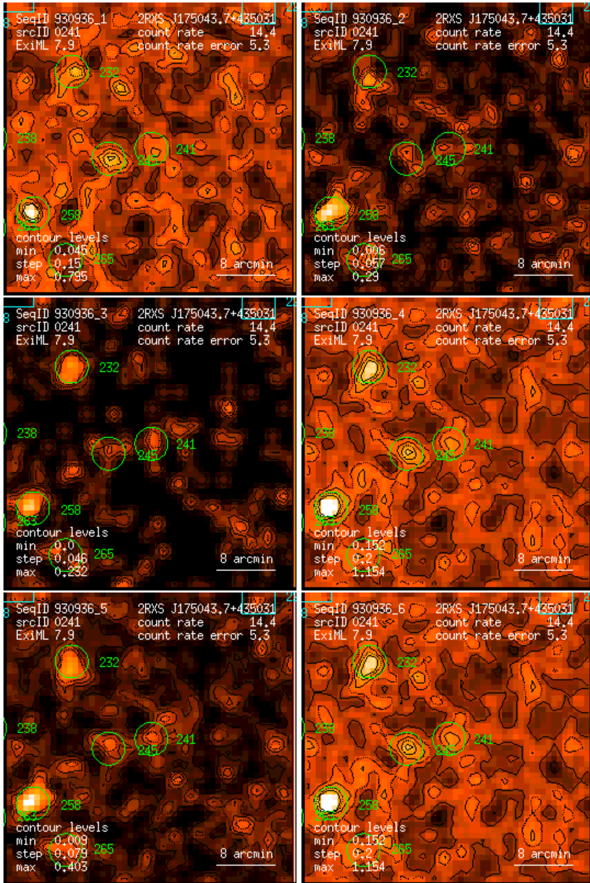
Figure 241: RASS 930936: detection 0241: band rate images, Gaussian filter: (1) PSPC channels 11 – 41, (2) 52 – 90, (3) 91 – 201, (4) 11 – 235, (5) 52 – 201, (6) 11 – 201. Broad band rates in counts/ks. Band rate contour levels in counts/ks/arcmin 2 .
