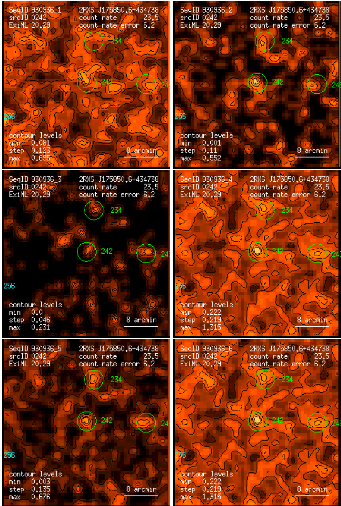
Figure 242: RASS 930936: detection 0242: band rate images, Gaussian filter: (1) PSPC channels 11 – 41, (2) 52 – 90, (3) 91 – 201, (4) 11 – 235, (5) 52 – 201, (6) 11 – 201. Broad band rates in counts/ks. Band rate contour levels in counts/ks/arcmin 2 .
