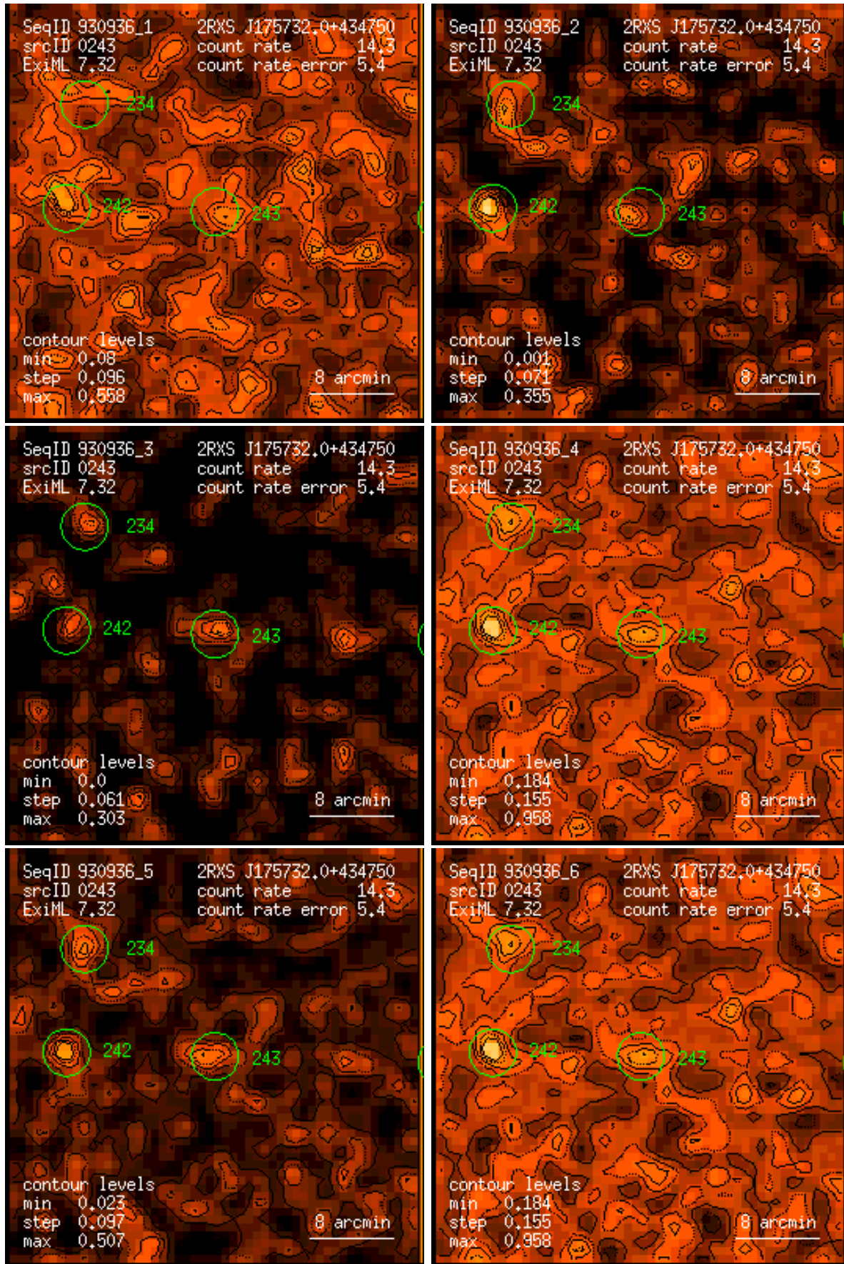
Figure 243: RASS 930936: detection 0243: band rate images, Gaussian filter: (1) PSPC channels 11 – 41, (2) 52 – 90, (3) 91 – 201, (4) 11 – 235, (5) 52 – 201, (6) 11 – 201. Broad band rates in counts/ks. Band rate contour levels in counts/ks/arcmin 2 .
